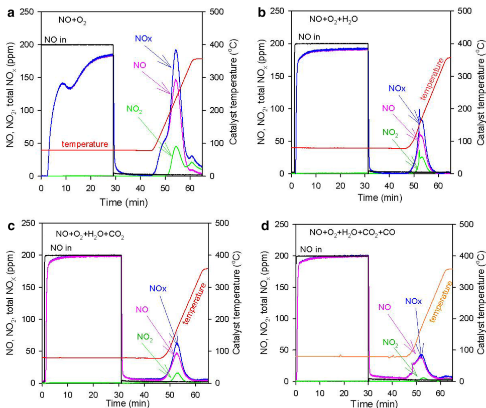
Fig. 9 TPD 1, 2, 3 and 4 (abbreviated in this study) over Pd/Ce/Al 2 O 3 catalyst using a NO+O 2 , b NO+O 2 +H 2 O, c NO+O 2 +H 2 O+CO 2 and d NO+O 2 +H 2 O+CO 2 +CO. For experimental details see Table 2
