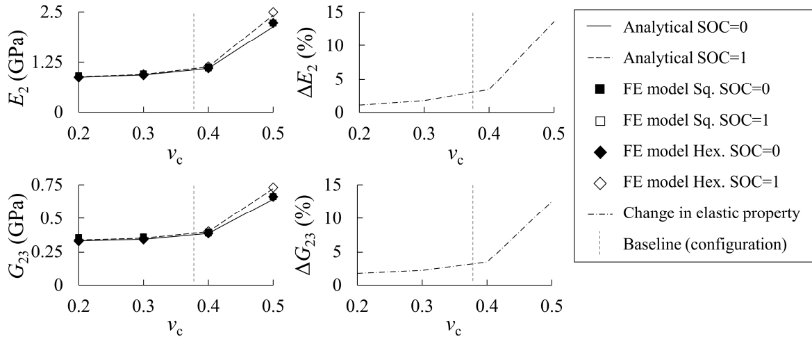
Fig. 6. Variation of effective elastic properties E_2 and G_{23} of the composite lamina at SOC=0 and SOC=1 with change in Poisson's ratio of coating \nu_c . Left figures: elastic properties. Right figures: difference in stiffness between discharged (SOC=0) and charged (SOC=1) state. Poisson's ratio of 0.38 corresponds to the baseline.
