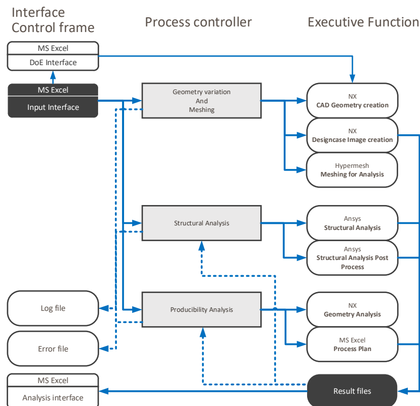
Figure 2.10 Engineering Workbench (EWB) working principles from (Heikkinen and Müller, 2015). In different studies mentioned in this thesis different ranges of analysis have been applied to a varying extent.
