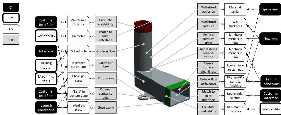
Figure 4.5 Original part geometry and functional decomposition, from (Borgue et al. , 2018)
