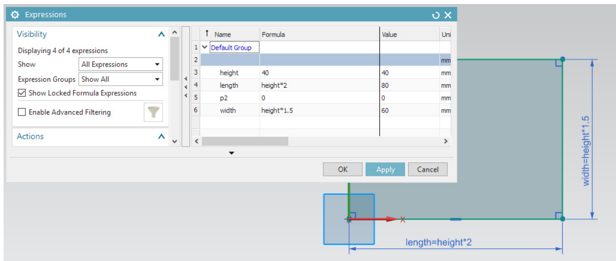
Figure 2.6 Screenshot from the CAD programme Siemens NX showing a parameterised sketch with relations between the dimensions length, height and width
