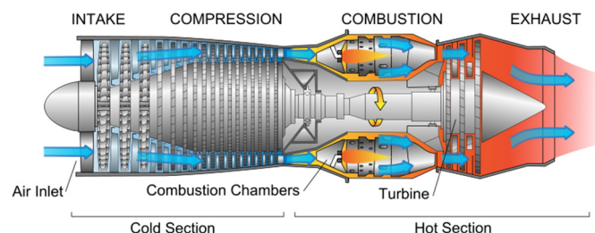
Figure 1.1 Diagram of a gas turbine jet engine. Air is compressed by the fan blades as it enters the engine, and it is mixed and burned with fuel in the combustion section. The hot exhaust gases provide forward thrust and turn the turbines which drive the compressor fan blades. 1
