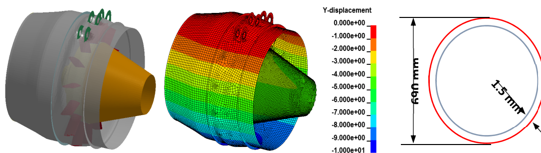
Figure 4.3 theoretical gap between TRS and cone due to thermal expansion mismatch CMC – Steel at 650°, simulations from the VITUM project performed by Swerea IWF.
