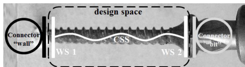
Figure 2.9 CCA model of a self-drilling screw and its environment, showing the CSS and working surface pairs (WS) from (Albers and Sadowski, 2014)
