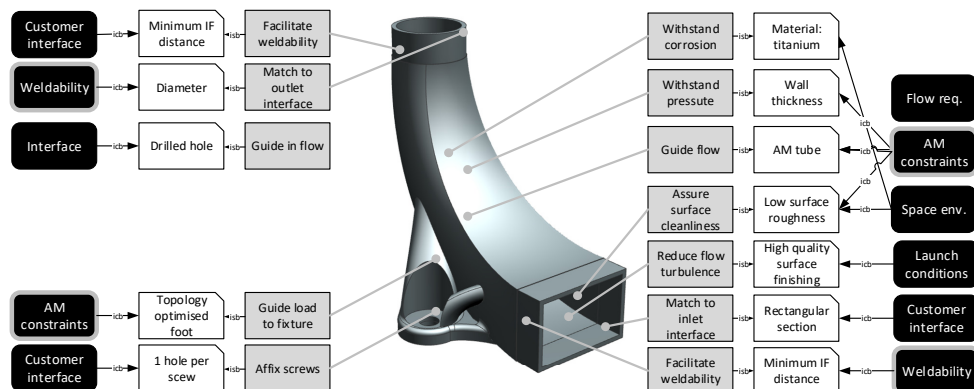
Figure 4.6 Redesigned part and associated function model, from (Borgue et al. , 2018)
