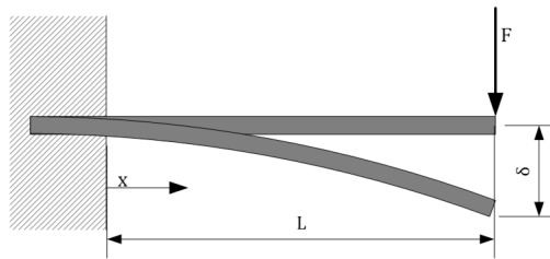
Figure 2.5 Physics model of the deflection of a beam
