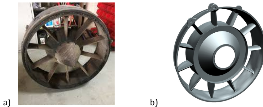
Figure 1.2 Turbine Rear Structure, a) from a Rolls Royce Conway jet engine from 1959 2 , b) rendering of a TRS as it is produced today.
