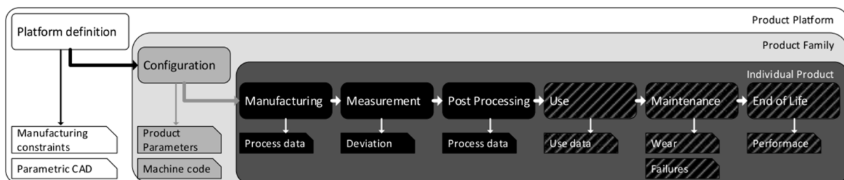
Figure 4.4 Process- and data flow in the demonstrator. Hatched elements have not been realised due to time and resource constraints. From (Müller, Panarotto, et al. , 2018)
