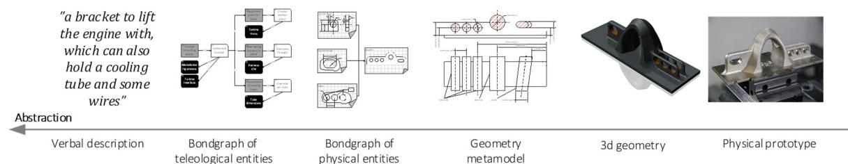
Figure 2.4 Abstraction levels of the same product "engine bracket" from paper B
