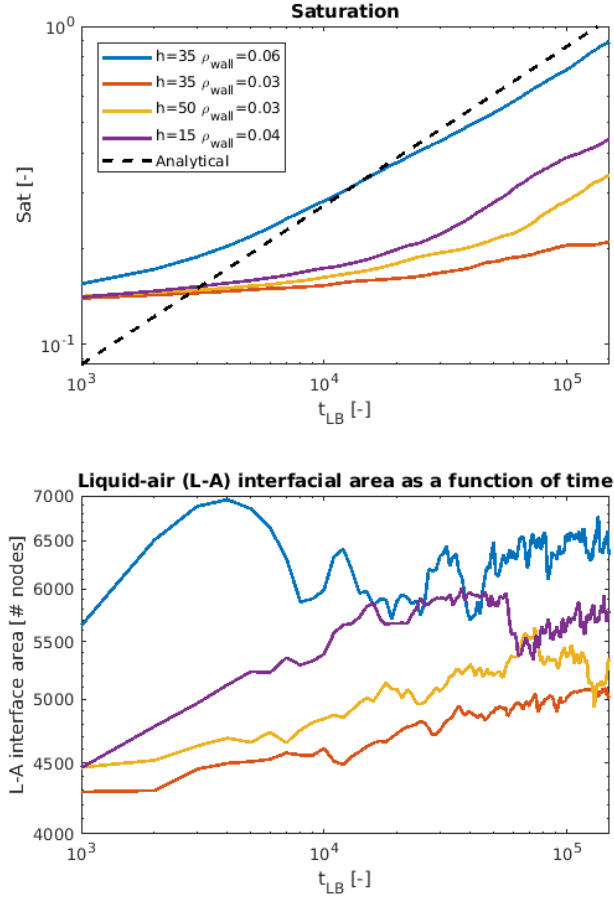
Figure 4.9: Saturation and liquid-air interfacial area over time.
