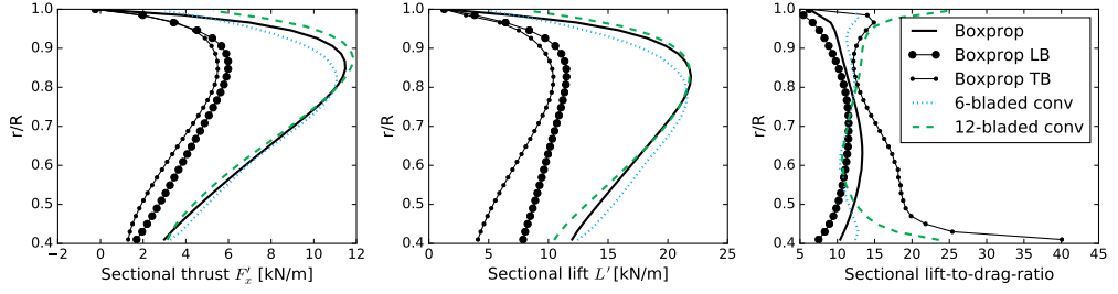
Figure 6.6.2: Sectional performance of the three optimized propellers.
