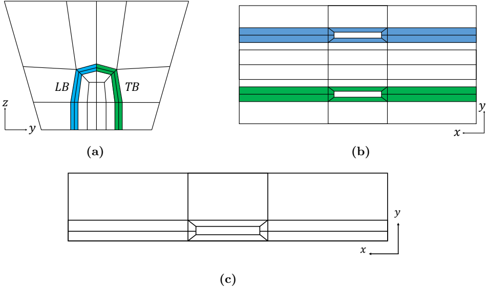
Figure 3.4.1: a) and b) Boxyprop blocking structure. Blue denotes the wake and O-grid blocks for the LB of the Boxyprop, while green is for the TB. c) The conventional propeller blocking structure.
