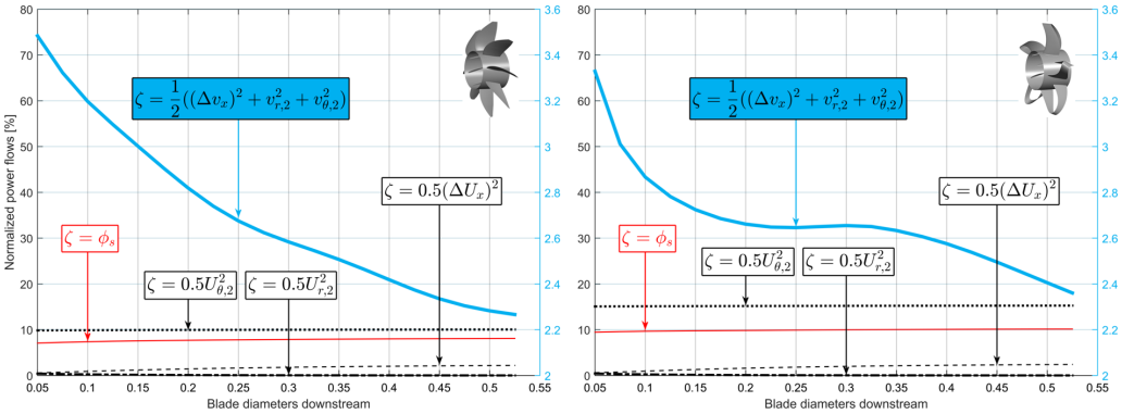
Figure 6.5.3: Power integrals \int \zeta d\ln for the loss terms of Eq. 6.5.3 for the conventional propeller (left) and the Boxprop (right). The loss terms have been normalized with shaft power and are plotted as a function of axial distance from the propeller trailing edge (TE at 75% radius). Note that the perturbation kinetic power level is plotted on the right-hand y-axis.
