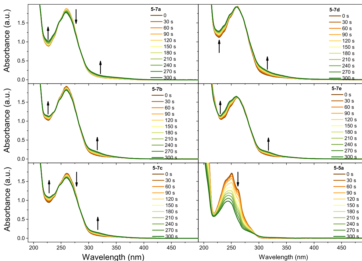
Figure 5-2: The UV-vis spectra of the 2-nitrobenzyl PPG-protected esters (5-7a-e) as well as phenylpropionic acid (5-5a) upon irradiation with a 254 nm. The arrow indicates the evolution direction of the absorption spectra with time. Reproduced from Paper IV, published under a Creative Common attribution (CC-BY) © American Chemical Society
