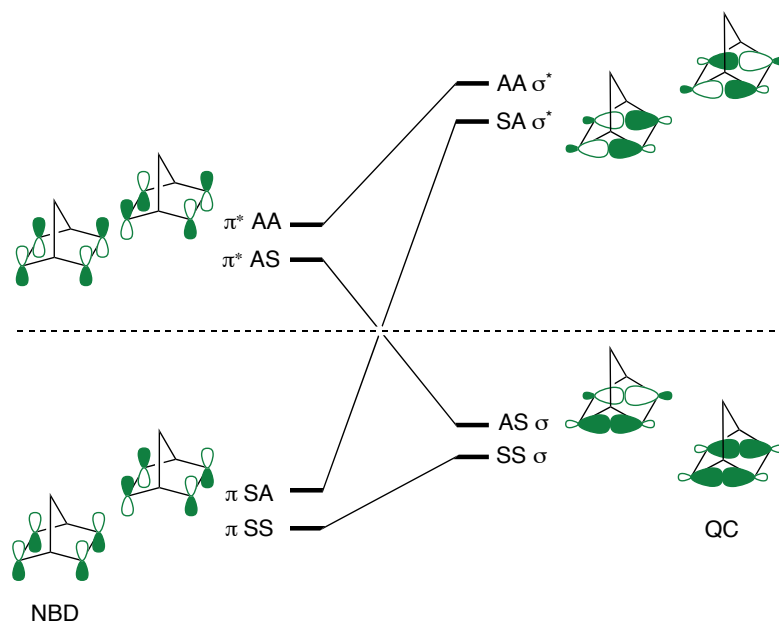
Figure 3-1 Correlation diagrams for norbornadiene-quadricyclane (NBD-QC) [2+2] photoisomerization based on the Woodward-Hofmann rule. Adapted from ref. 136 © 2003, John Wiley and Sons.
