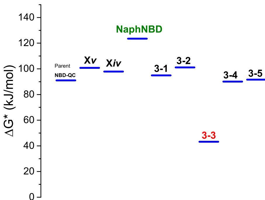
Figure 3-3: \Delta G^* values for various dimer NBD derivatives, as well as a monomer NBD derivative D with very long half-life (over 18 years) for comparison from ref. 167. Compound 3-3 with the shortest half-life (43.8 s) has the lowest \Delta G^* .
