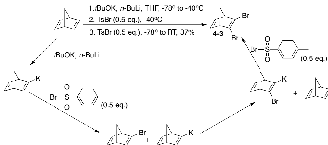
Scheme 4-3: The synthetic route to 2,3-dibromonorbornadiene ( 4-3 ) using tosyl bromide as a brominating agent.
