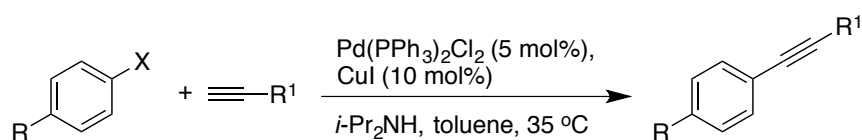
Scheme 4-4: Typical Sonogashira reaction conditions used in this thesis.
