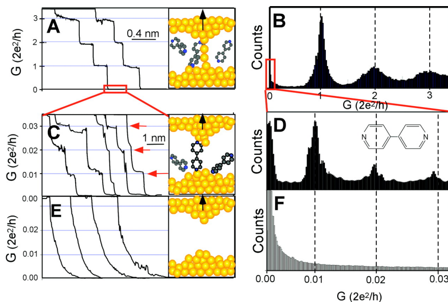
Figure 2-5: Schematic illustration of scanning tunnelling microscopy-break junction technique along with conductance traces and histograms of 4,4'-bipyridine. 47 Reproduced with permission ©2003, American Association for the Advancement of Science.
