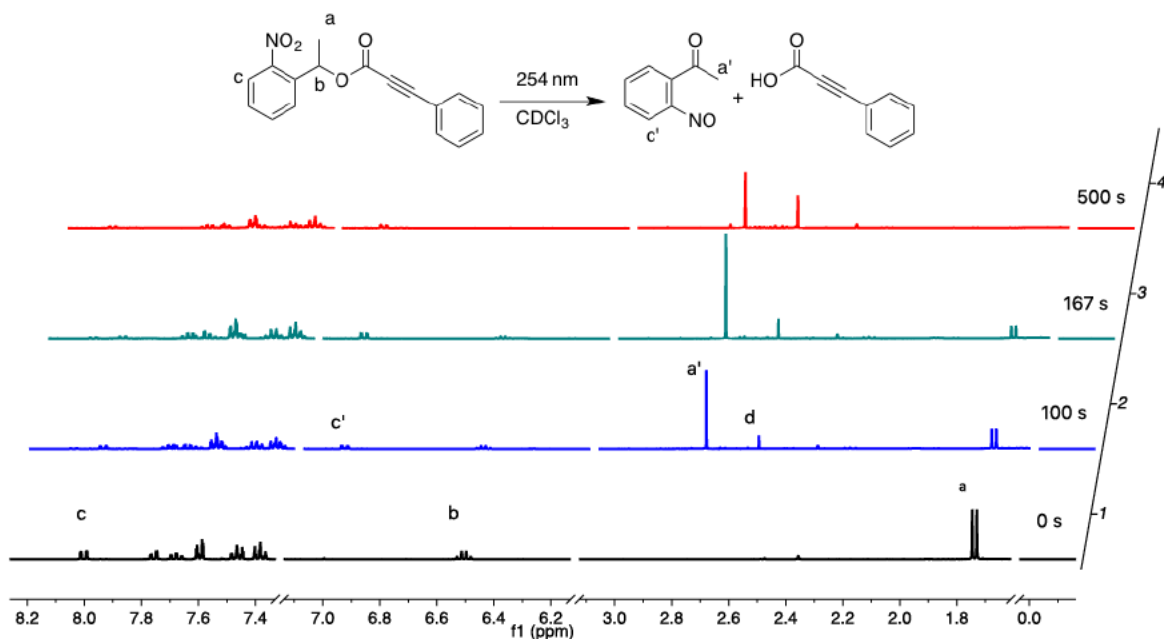
Figure 5-3: ^1\text{H-NMR} for the photodeprotection of compound 5-7b in a flow reactor chip at different flow rates, using a 254 nm handheld UV lamp. Upon photoirradiation new peaks a' , c' and d started to emerge, while peaks a and c disappear gradually. Reproduced from Paper IV, published under a Creative Commons attribution (CC-BY) © American Chemical Society
