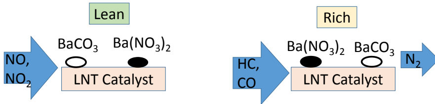
Figure 2.11: Simplified mechanism of lean \text{NO}_x trap shown during \text{NO}_x adsorption under fuel lean conditions (left) and \text{NO}_x reduction under fuel rich conditions (right).
