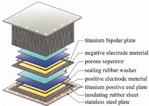
Figure 32. Bipolar design [130].
