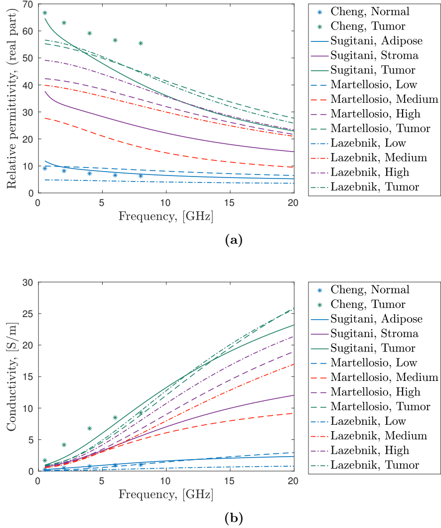
Figure 1.4: Dielectric properties as reported in several different studies, (a) relative permittivity and (b) conductivity. The tissues are grouped as: blue, adipose/low density; red, medium density; purple, high density; and green, tumor. Data retrieved from [50–54]. Reported standard deviations are omitted due to presentation reasons.
