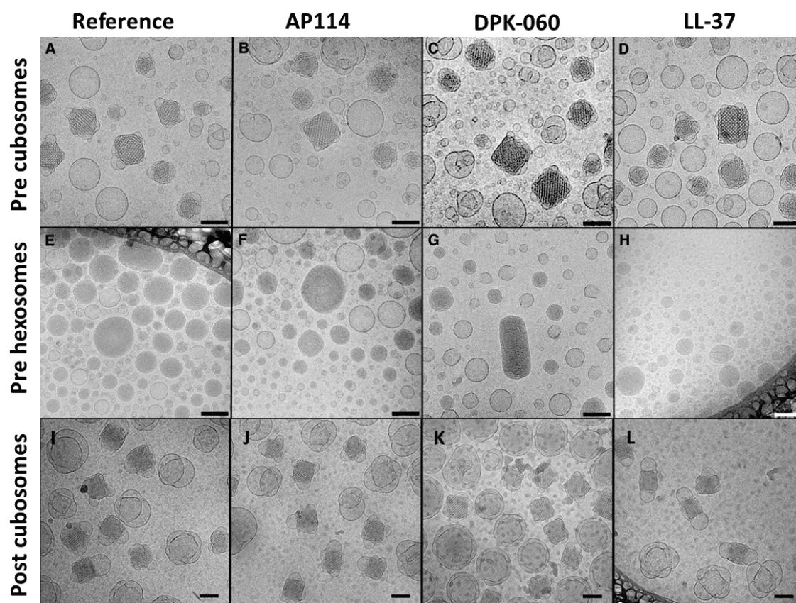
Figure 14. Cryo-TEM images of pre- and post-loaded LCNPs. Pre-loaded GMO-based cubosomes (A-D) and GMO/OA-based hexosomes (E-H) were loaded with 1 wt % AMP prior to dispersion, resulting in a final concentration of 500 µg/mL. Post-loaded cubosomes (I-L) contained 100 µg/mL AMP and the particle concentration was 10 mg/mL. Scale bars equal 100 nm.
