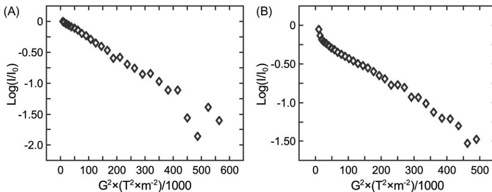
Figure 5. \text{Log}(I/I_0) plotted versus G^2 \times (T^2 \times \text{m}^{-2}) for pure particles (a) and a two-component system of free PEG and PEG-modified dye-doped silica nanoparticles (b), as measured by NMR-d. The first points in the two-component system represent a faster diffusing component, the free PEG, while the diffusion of the silica particles is captured by the less steep slope (further details are given in Figures S2–S3).
