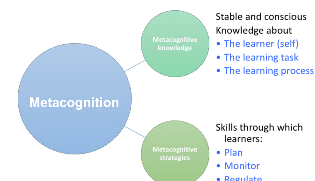
Fig. 2. Metacognition theory
