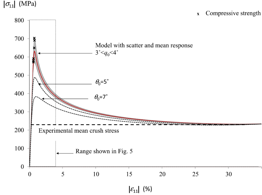
Figure 16: Evolution of kinking stress vs. experimental results for the HTS45/LY556 material system: Strength and mean crushing stress [50].
