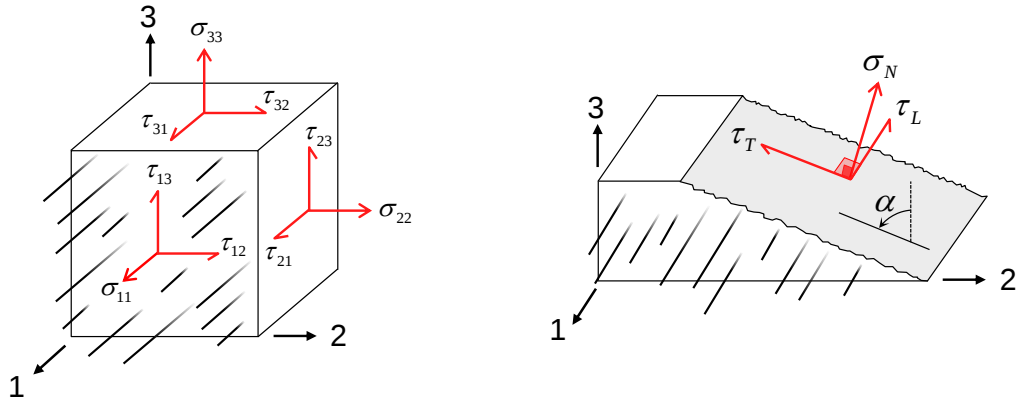
Figure 10: External stresses acting on a UD composite and (\sigma_N, \tau_L, \tau_T) stresses on a matrix failure plane.
