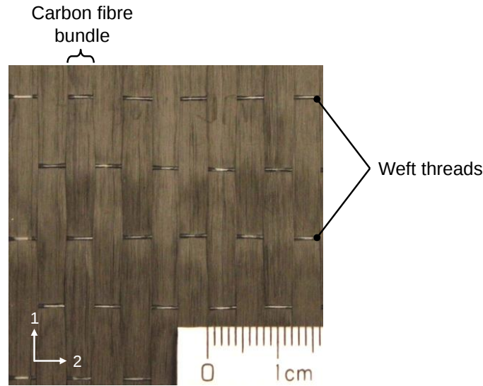
Figure 7: Photograph of the HTS45/LY556 uni-weave NCF reinforcement, from Paper A .
