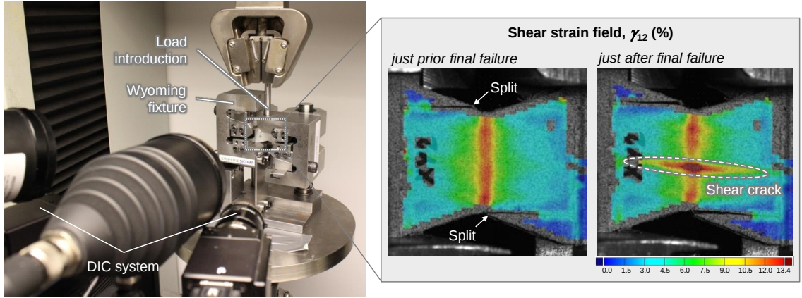
Figure 12: Shear strain field measured experimentally in a Iosipescu specimen, from Paper B .
