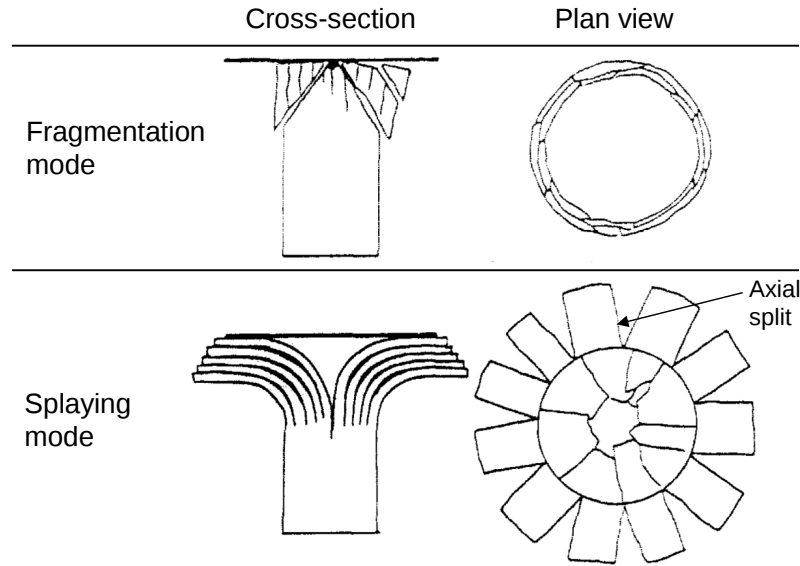
Figure 3: Schematic representation of the fragmentation crushing mode and the splaying crushing mode for a CFRP tube; after [10].
