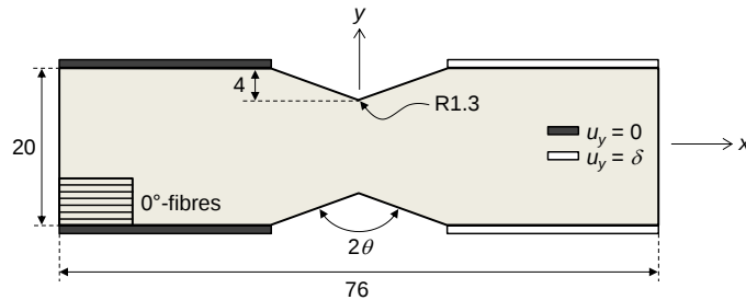
Figure 11: Iosipescu shear specimen (dimensions in mm).
