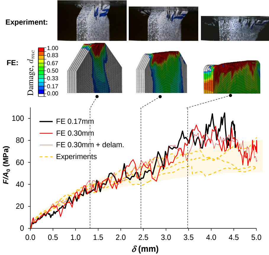
Figure 19: Experimental and numerical crushing response of the [45^\circ]_{10} arrow shaped coupons, from Paper E .
