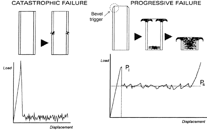
Figure 1: Catastrophic failure versus progressive failure (crushing) of a composite structure; after [8].
