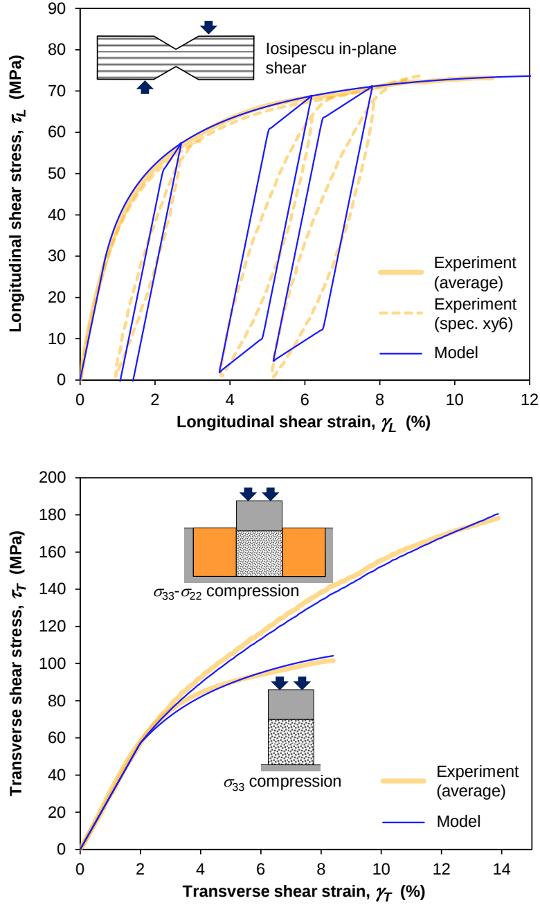
Figure 14: Calibration of the shear part of the ply-based damage model from experiments (longitudinal shear up, transverse shear down).
