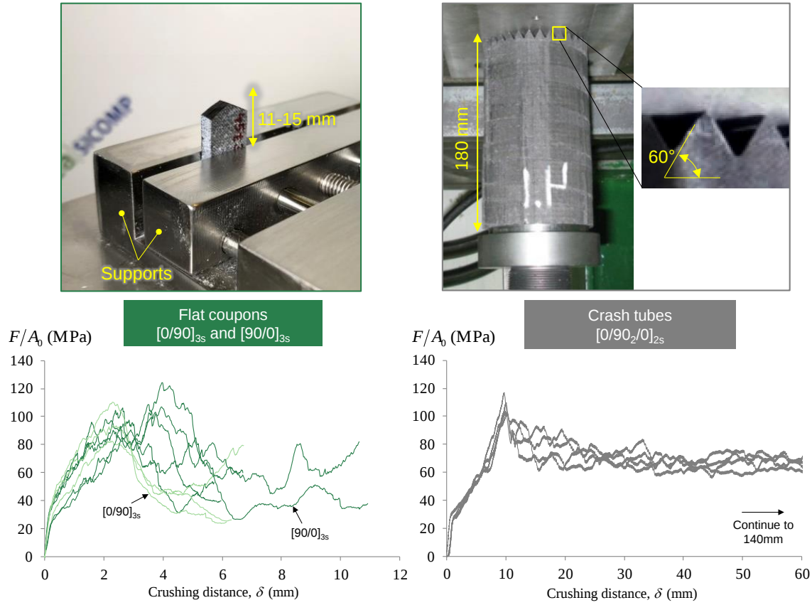
Figure 17: Results of quasi-static crush tests on cross-ply HTS45/LY556 laminates using small flat coupons and using larger crash tube structures.
