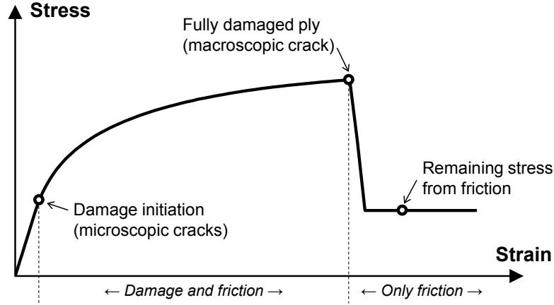
Figure 9: Representative stress–strain response for the material model combining damage and friction.
