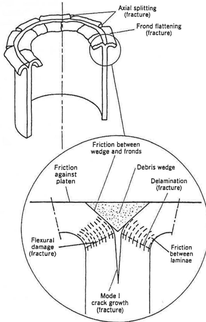
Figure 2: Schematic representation of the crush zone morphology for a CFRP tube subjected to axial loading [9].
