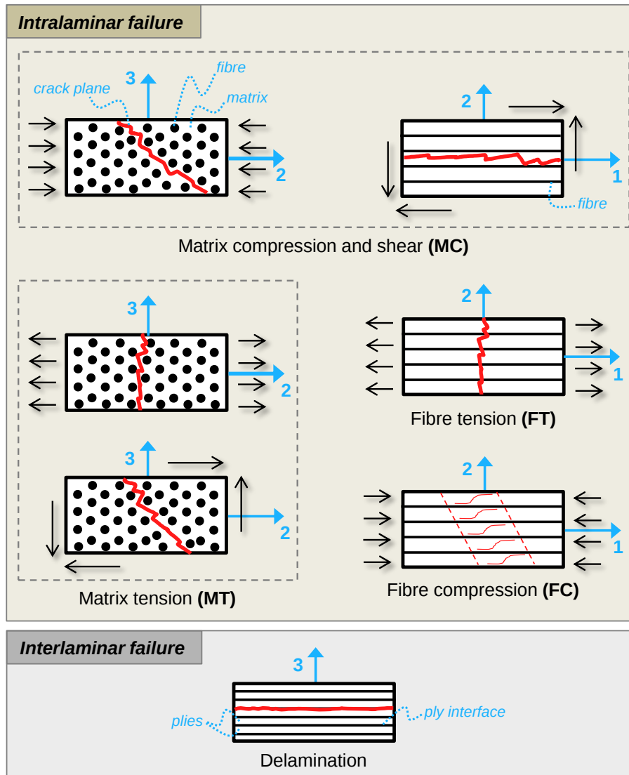
Figure 4: Energy dissipating failure mechanisms of continuous fibre composite materials in crash scenario.
