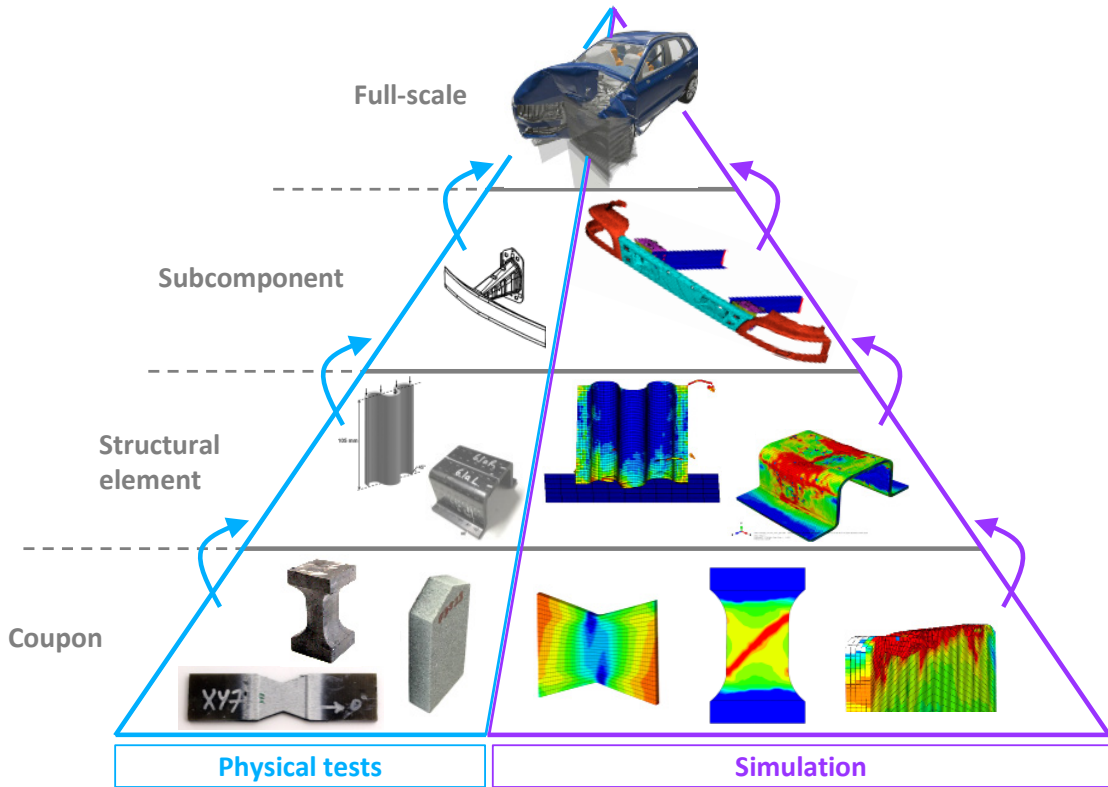
Figure 5: The building block approach applied to automotive composite crash structures.
