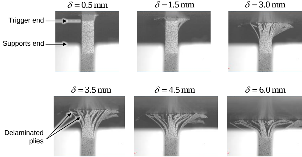
Figure 18: Edge of a [0/90]_{3s} crush coupon observed at different crushing distances \delta .
