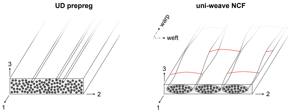
Figure 8: Illustration of a UD prepreg ply and a uni-weave NCF ply with weft threads.
