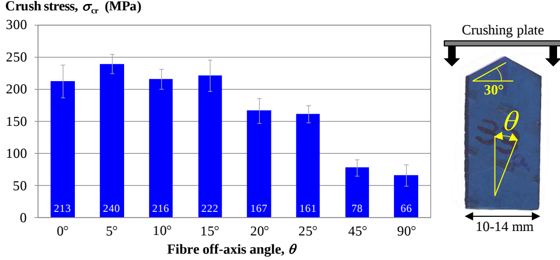
Figure 15: Average crush stress in UD HTS45/LY556 flat coupons with different off-axis angles, from Paper D .
