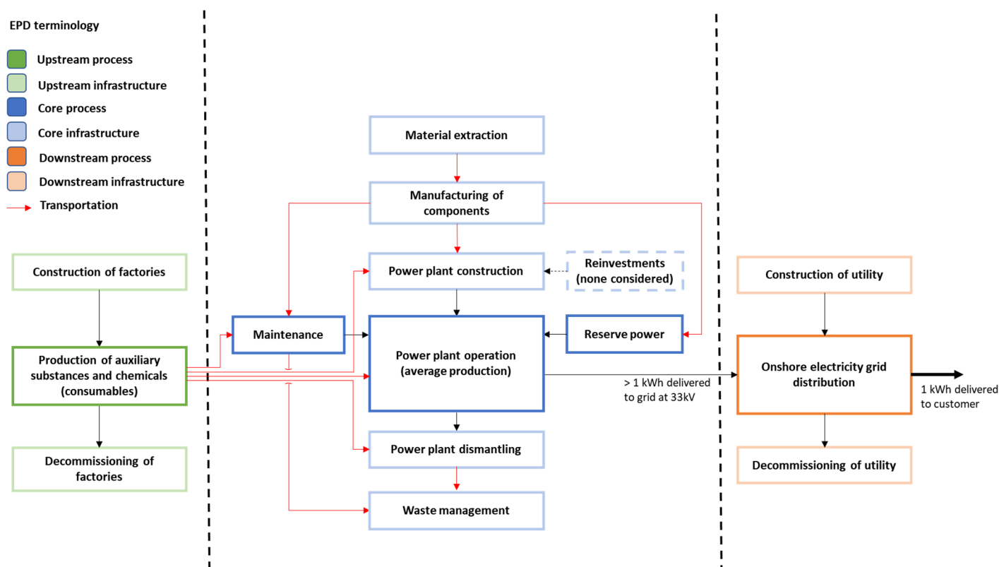
Figure 3. Overview flowchart of the inventory model for the DGU tidal current power plant based on the PCR.
