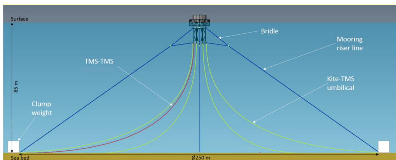
Figure 10. Illustration of Tidal Marine Substation buoy (Minesto).
