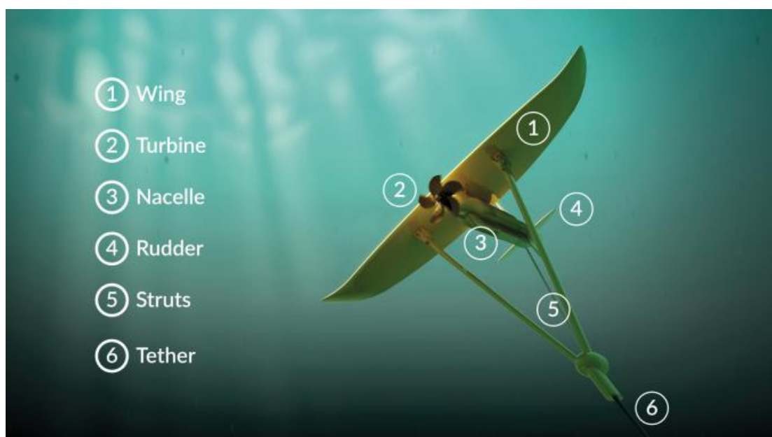
Figure 5. Illustration of the kite and its components (Minesto).
