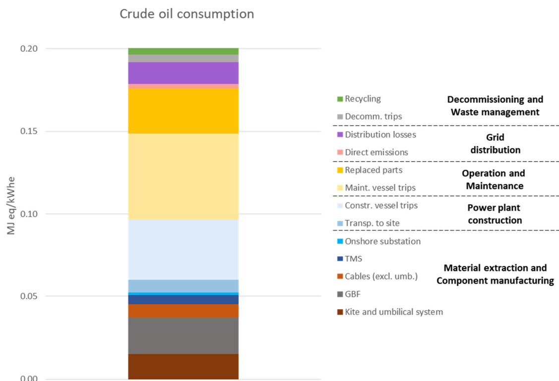
Figure 16. Contribution to crude oil demand by life cycle stages.
