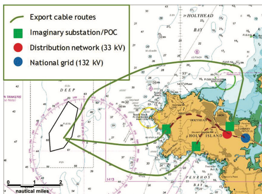
Figure 11. Options for offshore and onshore export cable routes (Minesto). The path with the shortest offshore export cable (middle) has been modelled in this study.
