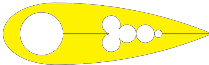
Figure 6. Cross-section view of a tether fairing, showing the spacing for the rope and cables (Minesto).
