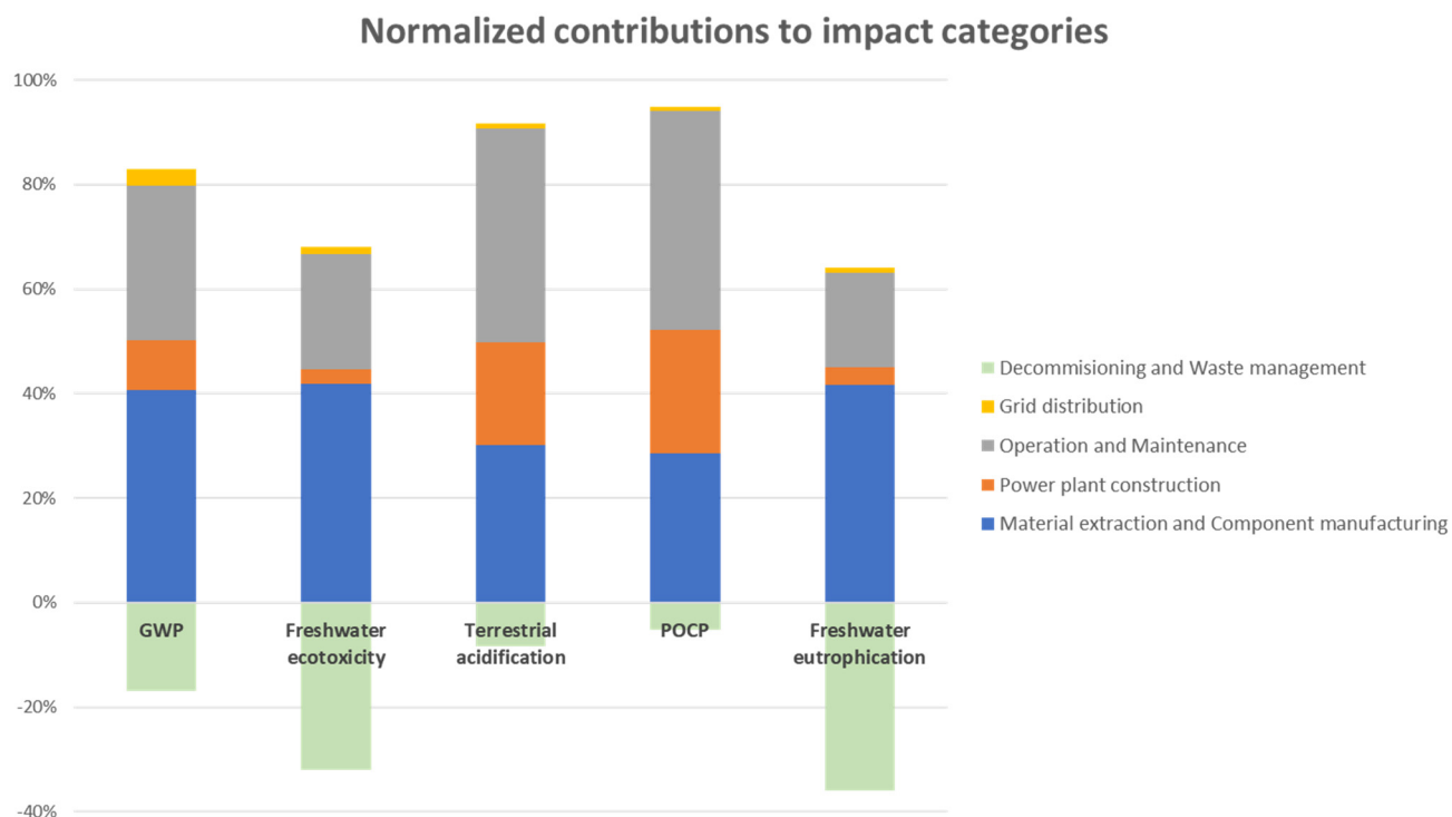
Figure 13. Overview of some assessed impact categories normalized to 100%, for the Base case scenario. The bar segments represent the different life-cycle stages. Processes contributing less than 1% are excluded.
