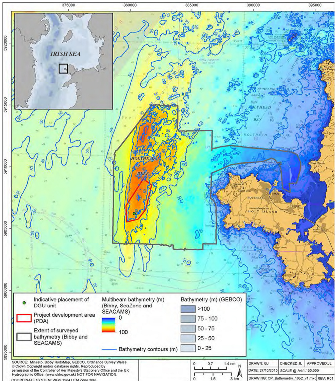
Figure 2. Map of the Holyhead Deep site for the DGU power plant. (The green circle indicates only the location of the first kite.) (Minesto, 2016).
