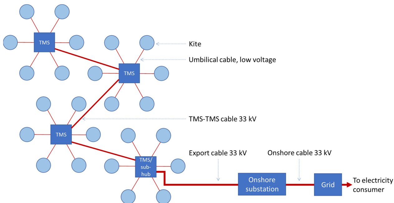
Figure 4. Schematic outline of the DGU tidal current power plant model assessed in this LCA.
