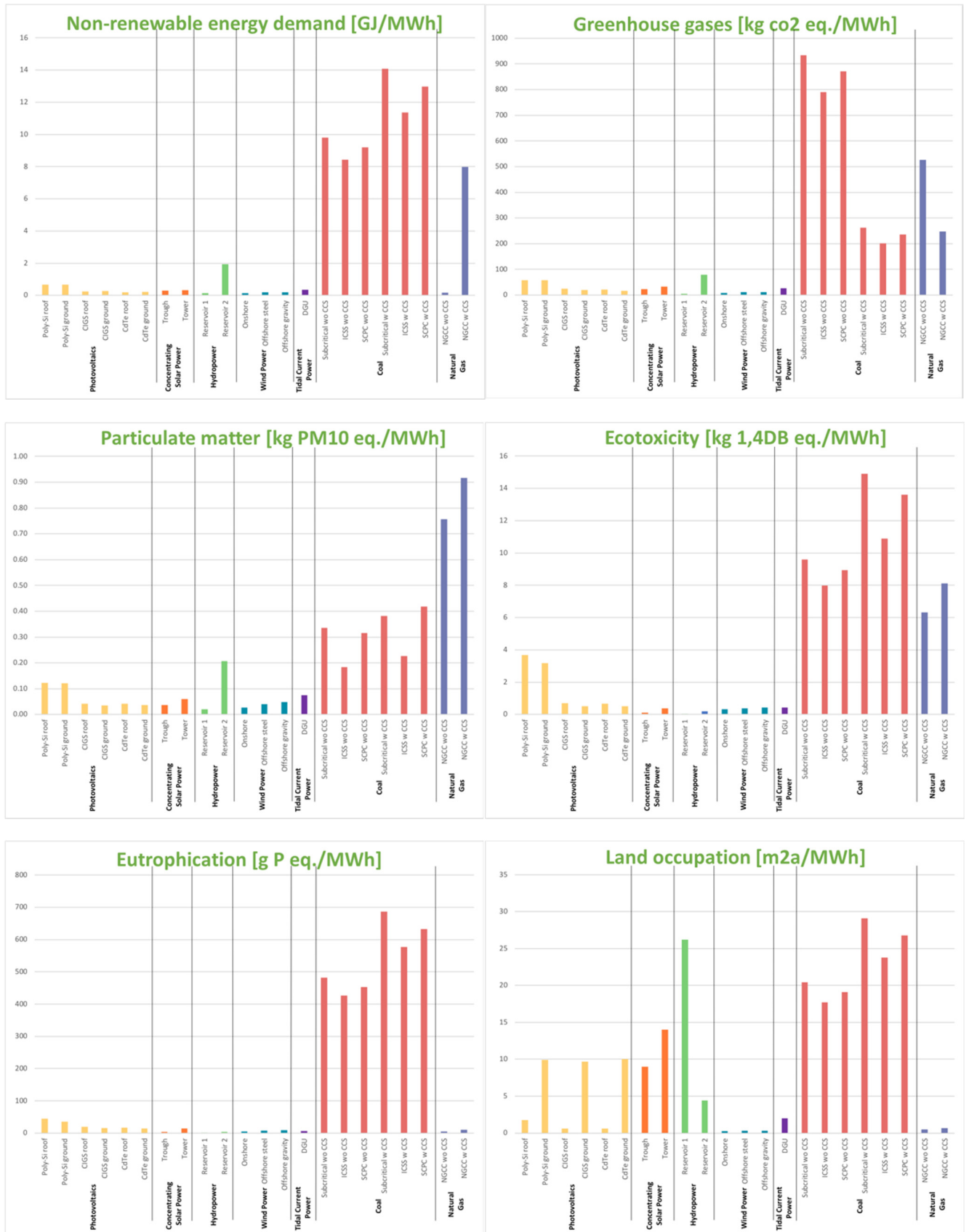
Figure 24. Impact on Land occupation, Non-renewable energy demand, Greenhouse gases (GWP), Freshwater eutrophication, Freshwater ecotoxicity, and Particulate matter formation. Comparisons of the DGU tidal power plant (purple – Base case) with the mean value of wide range of electricity generation technologies reported in H14.
