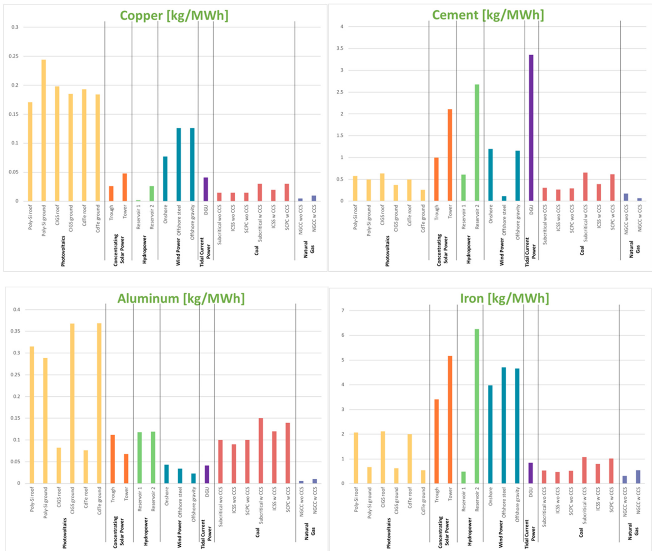
Figure 23. Material requirements in kg/MWh (or g/kWh). Comparison of the DGU tidal power plant (purple – Base case) with the mean value of wide range of electricity generation technologies reported in H14.
