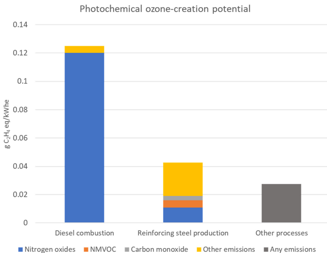
Figure 21. Impact on POCP in g C 2 H 4 eq/kWhe, contributions from processes and emissions (Base case). Processes contributing less than 1 % are aggregated into “Other processes”.
