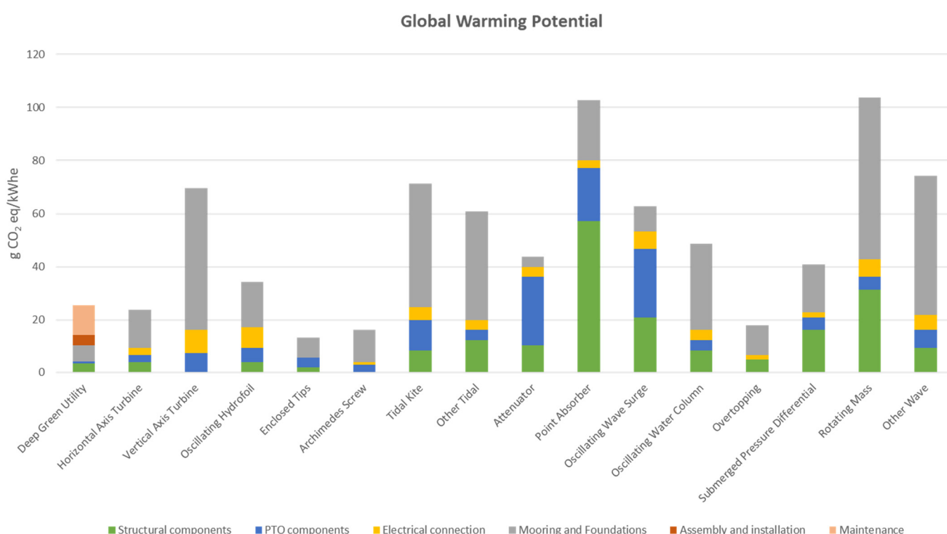
Figure 25. Impact on GWP. Comparison of the DGU tidal power plant (Base case) with other ocean-based electricity generation technologies reported by Uihlein (2016).
