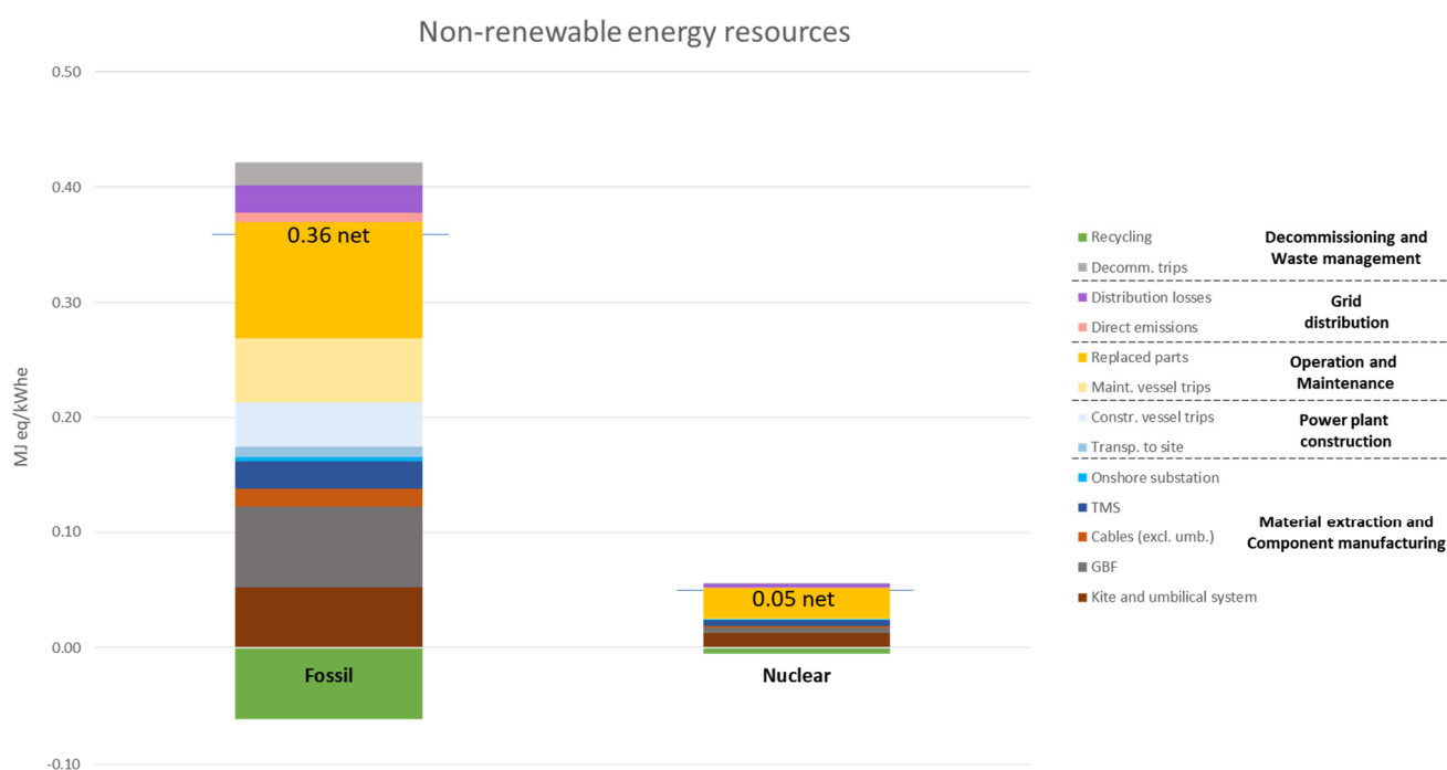
Figure 15. Non-renewable energy resources demand by different life cycle stages. The net demand is shown in numbers.
