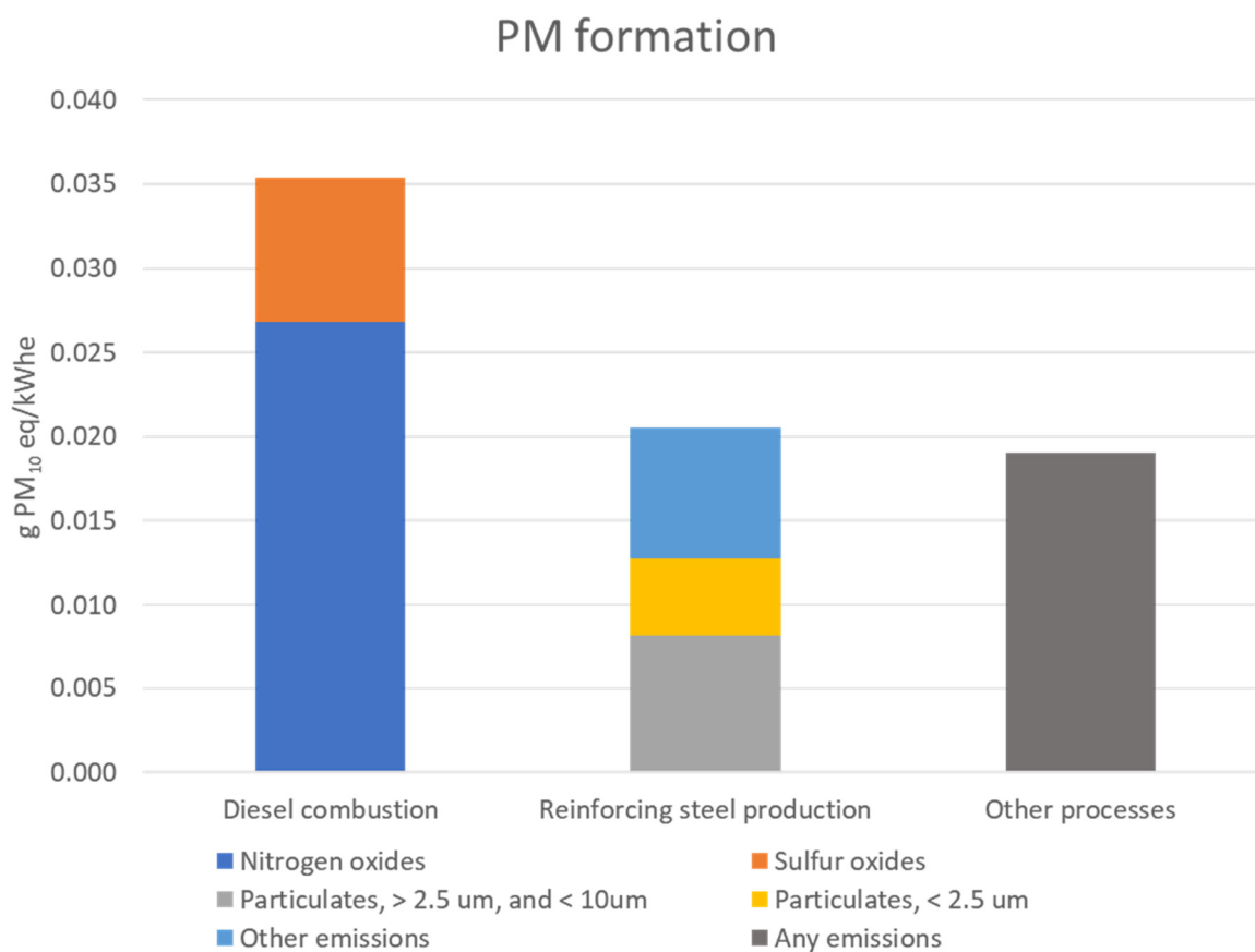
Figure 22. Impact on PM formation in g PM 10 eq/kWhe, contributions from processes and emissions (Base case). Processes contributing less than 1 % are aggregated into “Other processes”.
