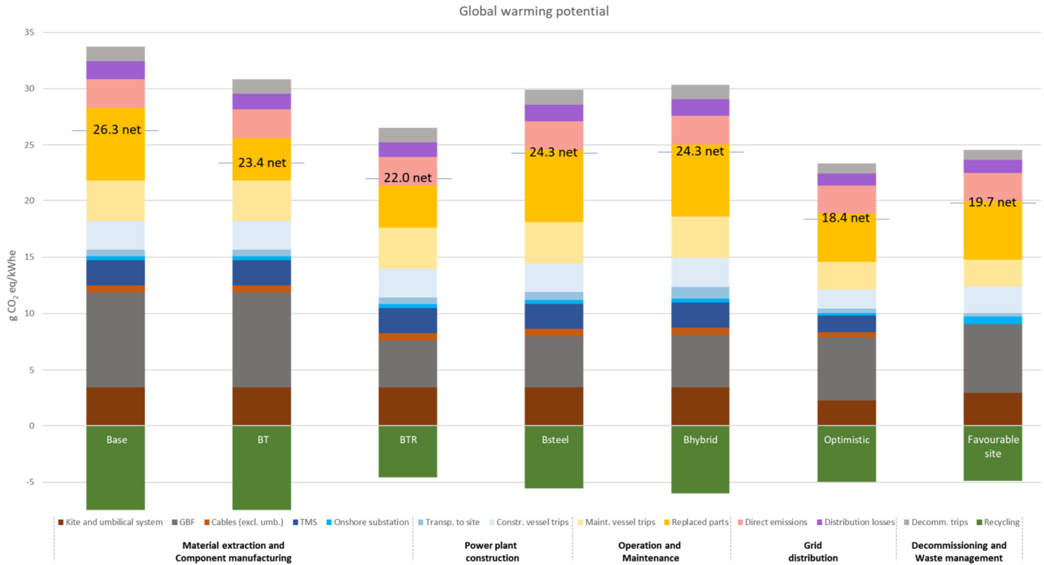
Figure 17. Impact on global warming potential g CO 2 eq/kWh for 7 of the scenarios defined in 4.1.2.1. The material yields from recycling copper and steel are credited as avoided impacts from producing virgin materials. The net impact is shown in numbers.
