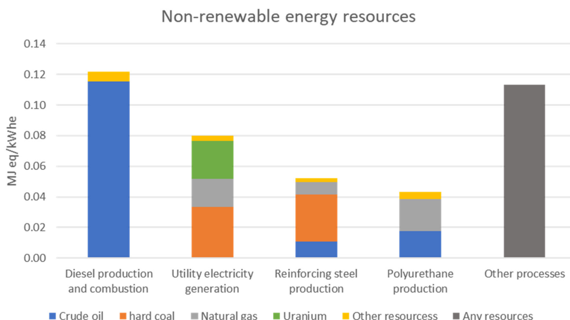
Figure 14. Non-renewable energy resources - fossil in MJ eq/kWhe, contributions from processes and resources (Base case). Processes contributing less than 1 % are aggregated into "Other processes".
