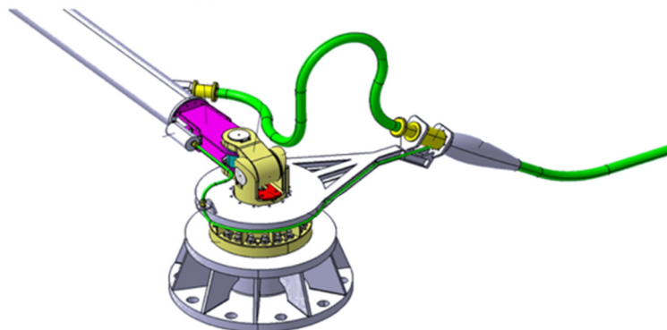
Figure 7. illustration of the Bottom joint (Minesto).
