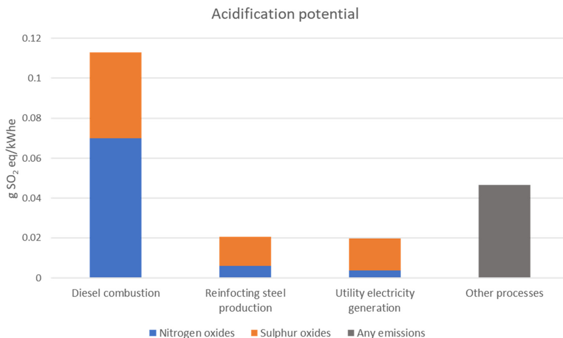
Figure 18. Impact on acidification potential in g SO 2 eq/kWhe, contributions from processes and emissions (Base case). Processes contributing less than 1 % are aggregated into “Other processes”.
