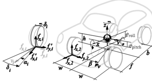
Figure 1. Vehicle model and coordinate system definition i \in \{1,2,3,4\} = \{FL, FR, RL, RR\} .
