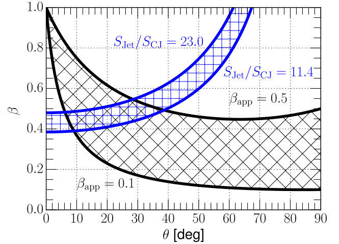
Fig. 10. Possible range of M87 jet viewing angles and jet speeds (in units of c ) that satisfy the measured jet-to-counter-jet ratio R and our assumptions of the value of \beta_{\text{app}} at the core separation of 0.2–0.5 mas. The cross and vertical hatches show allowed ranges of the parameters for R and \beta_{\text{app}} . Only the overlapping region is physically allowed under the assumptions outlined in Sect. 4.4.
