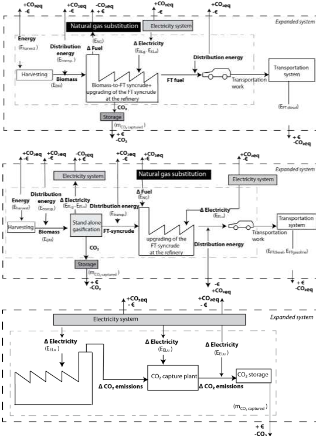
Figure 5-4. System boundaries for the systems analysis of the net annual profit and the GHG emissions.
