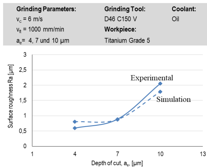
Fig. 26. Surface roughness versus depth of cut, a_e
