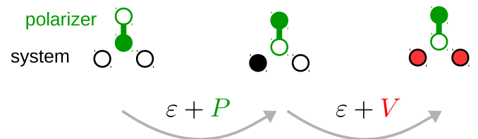
FIG. 1. A double-dot system (horizontal, black) with a nearby double-dot polarizer (vertical, green). Whereas the system can host either 0, 1, or 2 electrons with interaction V , the polarizer contains only one electron that can be excited at an energy cost P . The system acquires effective attractive electron interaction when the addition of the second electron costs less energy than adding the first. This is realized here for P > V : when the first electron excites the polarizer [beyond the orbital energy \varepsilon defined in Eq. (11)], the second electron only needs to overcome the lower electron repulsion energy.
