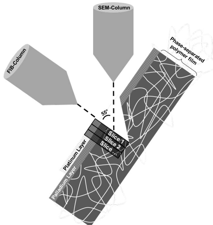
Figure 4. The setup of focused ion beam combined with scanning electron microscope and the specimen. The incident angle of the electron beam and the ion beam is 90^\circ and 55^\circ , respectively, in order to perform milling an imaging immediately after each other.
