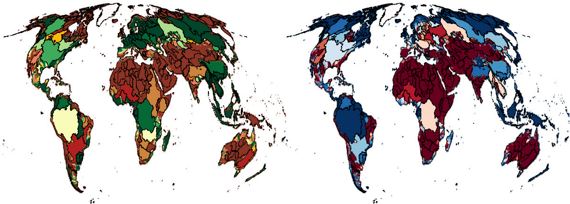
FIGURE 5 Limitation of bioenergy crop plantations due to available renewable water resources at basin level under the “Food & Nature” scenario
