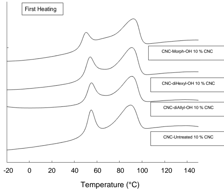
Figure 20: DSC endotherms for the composites containing surface-treated and untreated CNC (10 weight-%).
