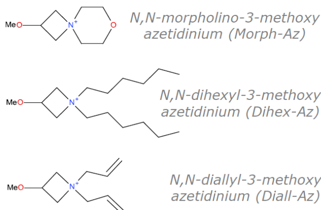
Figure 5: Schematic outlines of the molecular structures of the salts.
