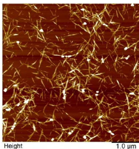
Figure 2: AFM micrograph of a dried CNC network (Moberg et al. 2017).
