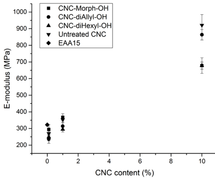
Figure 15: The elastic modulus of the composites as a function of the CNC-content.
