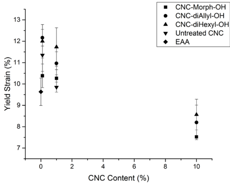
Figure 16: The yield strain of the composites as a function of the CNC-content.
