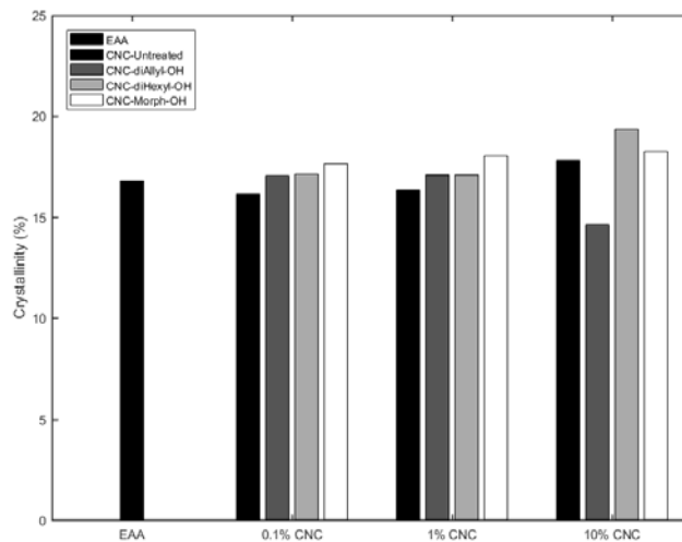
Figure 21: The total crystallinity of the unfilled EAA and the CNC-containing composites.
