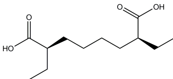
Figure 3: EAA molecular structure with alternating ethylene repetitive units and acrylic acid sections.
