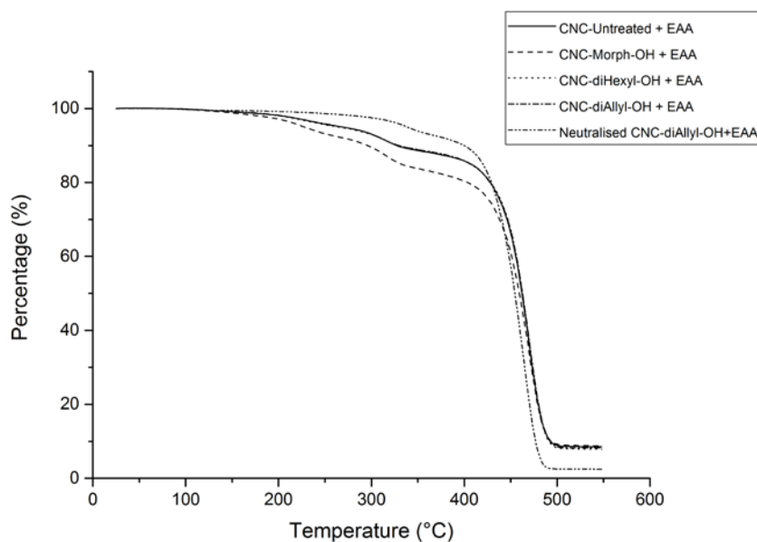
Figure 13: Thermogravimetric curves showing the thermal degradation of the composites containing unmodified CNC, the azetidinium-grafted CNC and a model sample produced under neutralised conditions.
