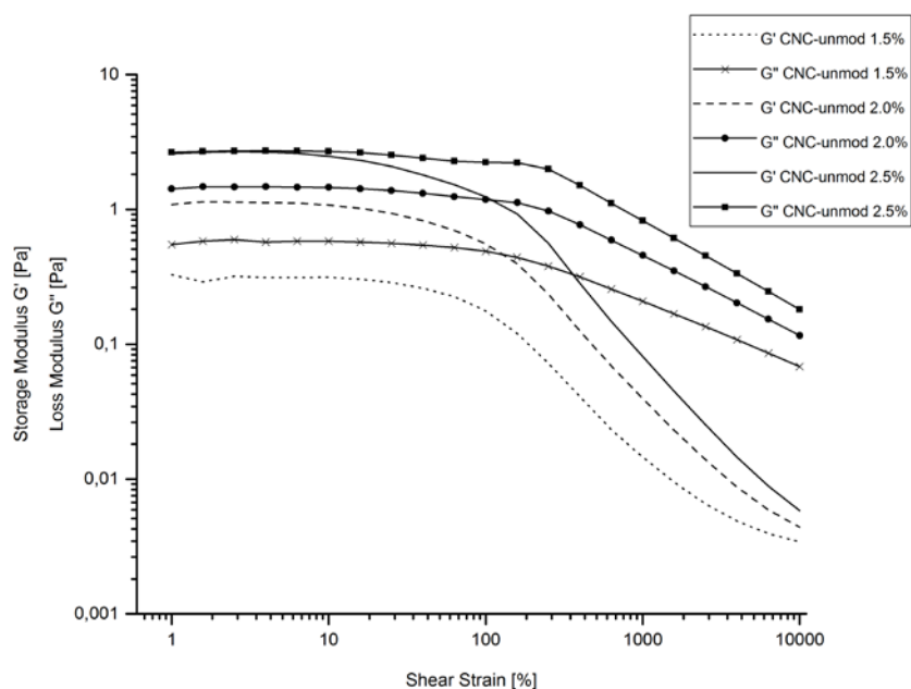
Figure 10: The dynamic mechanical moduli at a frequency of 1 Hz and 25 °C as functions of the applied shear strain amplitude for aqueous dispersion containing different concentrations of untreated CNC. At a concentration of 2.5 weight-% CNC, the storage and loss moduli coincide over a substantial part of the applied shear strain region.
