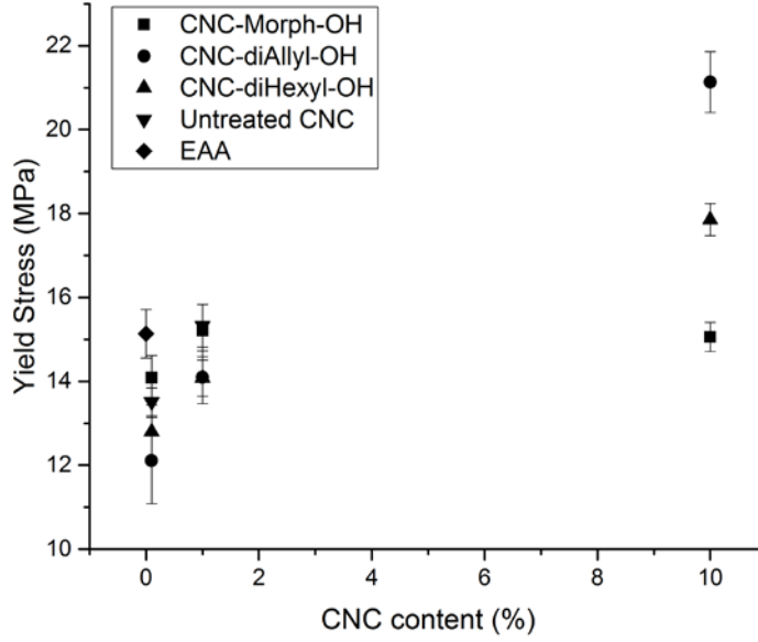
Figure 17: The yield stress of the composites as a function of the CNC-content.
