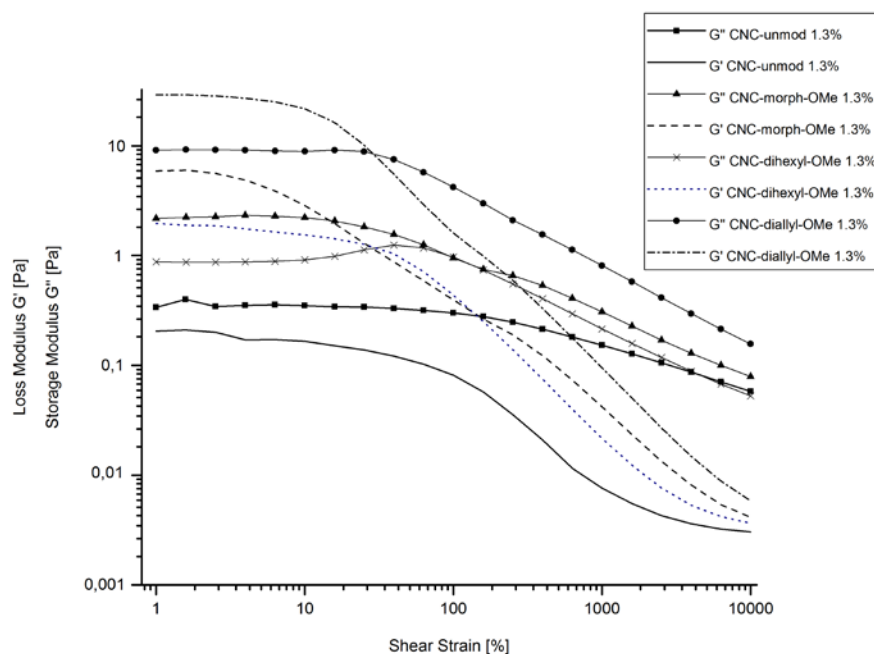
Figure 9: Dynamic-mechanical properties (at a frequency of 1 Hz) of the CNC dispersions as a function of the applied strain amplitude at 25 °C. The CNC-concentration was 1.3 weight-%.
