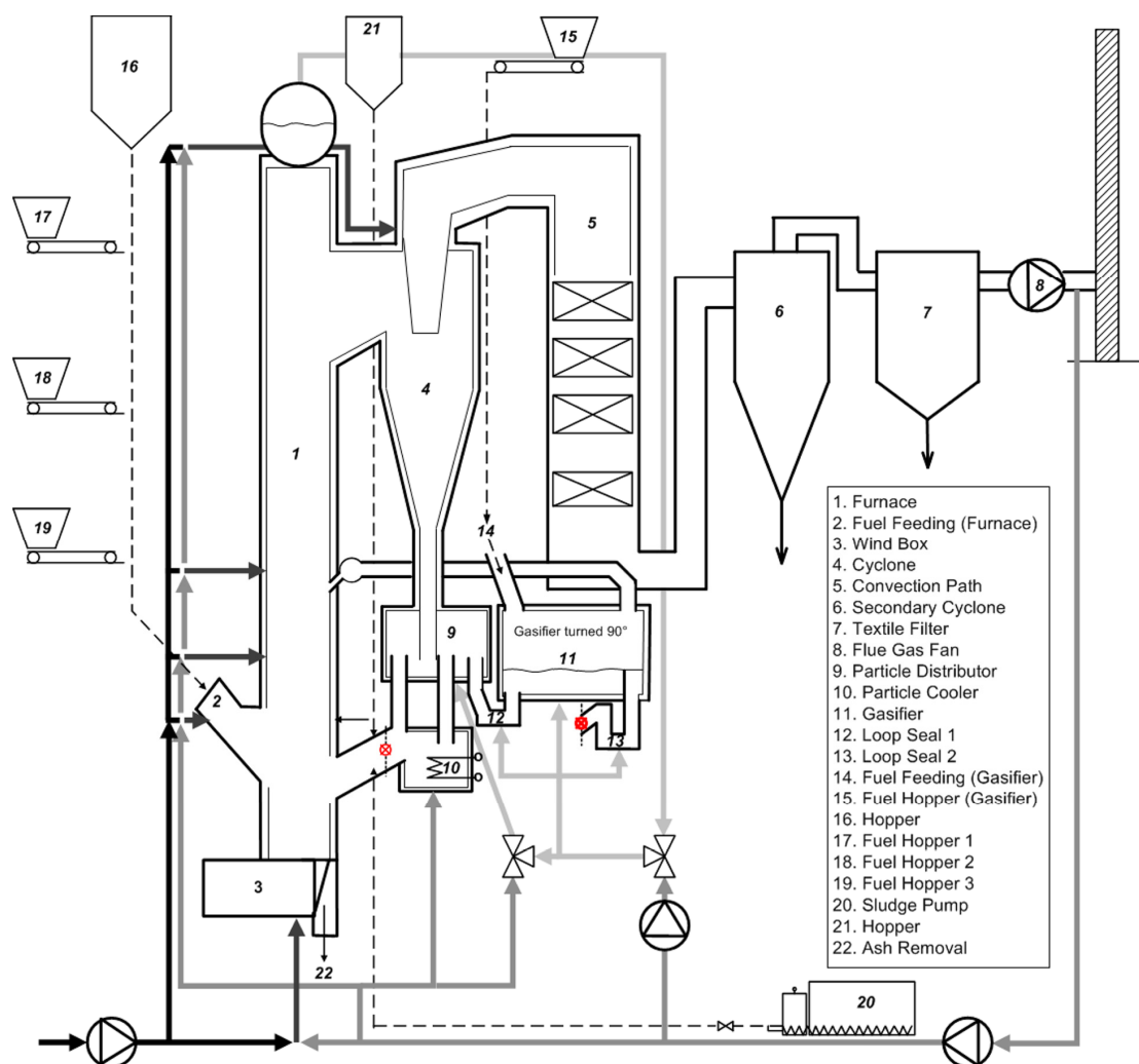
Figure 5.4. Schematic of the Chalmers DFBG system.
