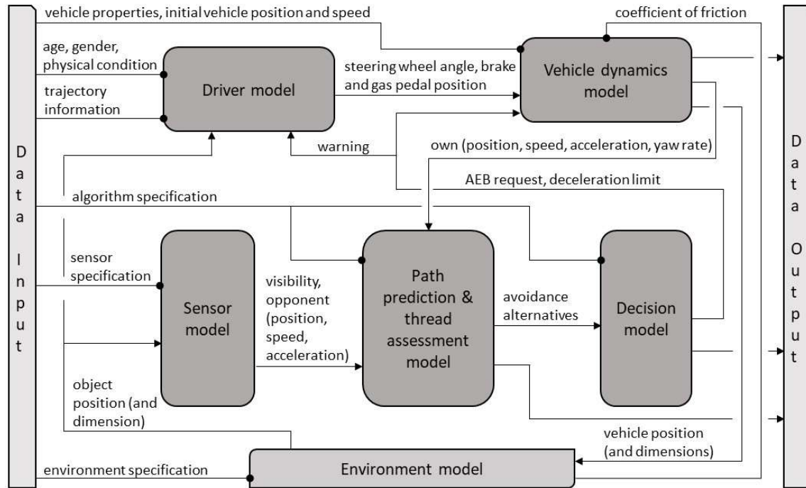
Figure 5: Data flow between simulation models. Parameter-flow (time-independent) is marked with —● and variable-flow (time-dependent) with —>.
