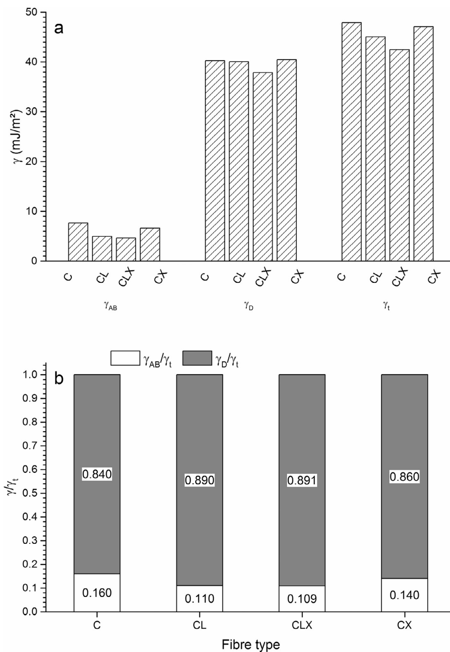
Fig. 6. Surface energies as obtained by IGC (a) and share of polar and dispersive components in the total surface energy (b) for all fibre types.
