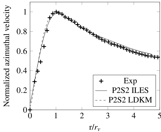
Figure 4.9: Variation of the normalized azimuthal velocity at the vortex core region, the velocity is normalized by u_\theta = 6.7m/s , z/C = 1.14
