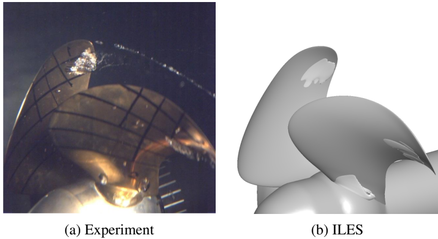
Figure 5.16: Side view of numerical predictions vapour Iso-surfaces (50 %) and experimental snapshot, propeller A.
