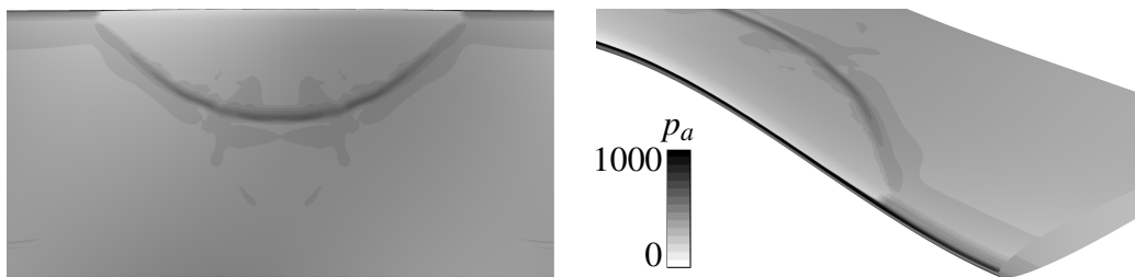
Figure 5.2: Added Pressure to the threshold pressure due to the viscous effects for cavitation around Twist11.
