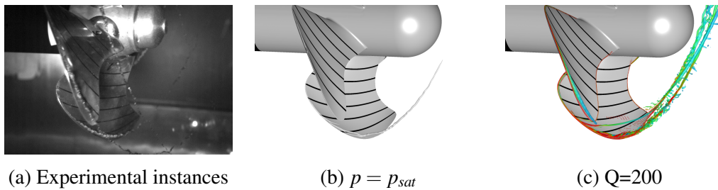
Figure 7.13: Comparisons between experimental instances and numerical predictions in the wetted flow conditions, propeller C, OW, J=1.26 , \sigma = 2
