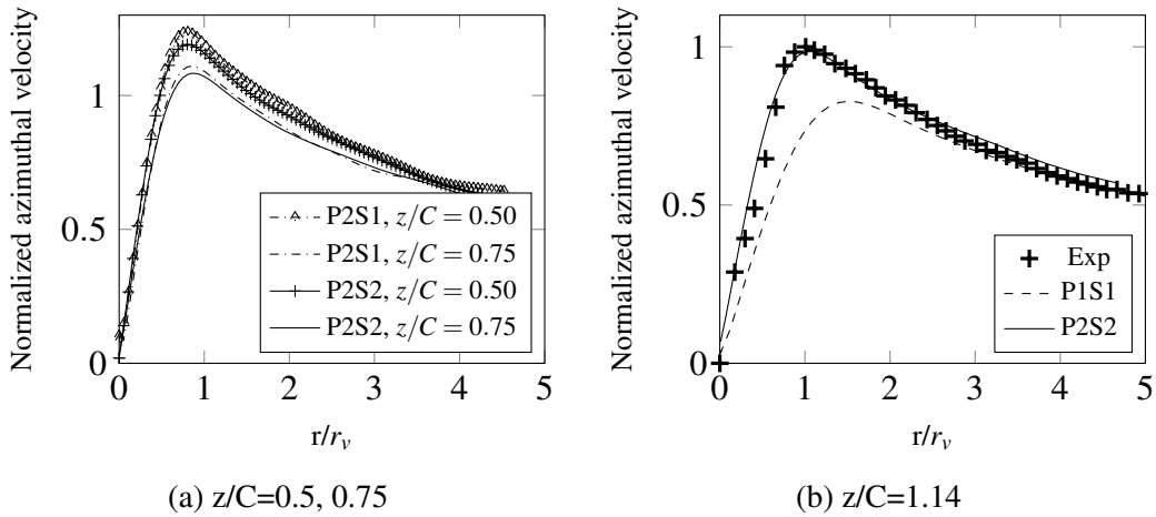
Figure 4.3: Variation of the normalized azimuthal velocity at the vortex core region, ILES, wetted flow results. The vortex core radius is normalized by r_v = 1.1mm , and the velocity is normalized by u_\theta = 6.7m/s .
