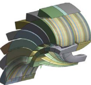
LEMCO TEC: Involute spiral arrangement of IC for space optimization Source: Zhao et al., 2015
