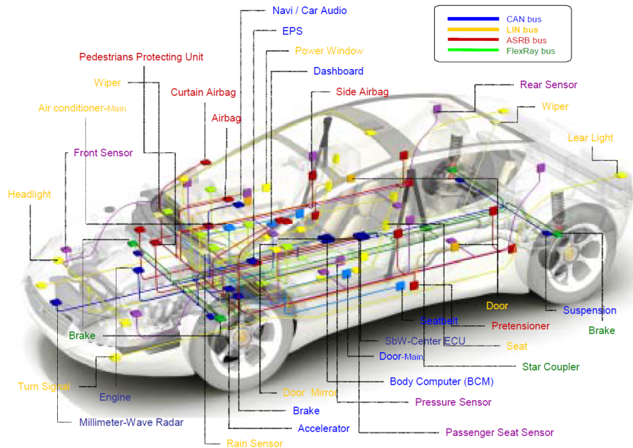
Figure 1.1: Example of a vehicular ECU network [7].
