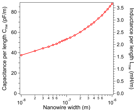
Figure 6.1: Simulated capacitance per length for nanowire widths ranging from 1 \mu\text{m} down to 10 nm. The right axis corresponds to the minimum required inductance per length to verify Z_{nw} > R_Q .
