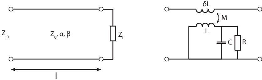
Figure 3.3: (left) Portion of transmission line of length l loaded with an impedance Z_L (right) Half-wavelength resonator inductively coupled to a transmission line. Energy is exchanged through the mutual inductance between the probing line and the resonator.
