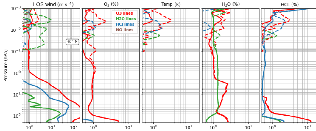
Figure 10. Spectroscopic-induced errors in LOS wind, temperature, O_3 , H_2O and HCl retrievals (see panel titles). The full lines (dashed lines) show the nighttime (daytime) conditions at 60^\circ N .
