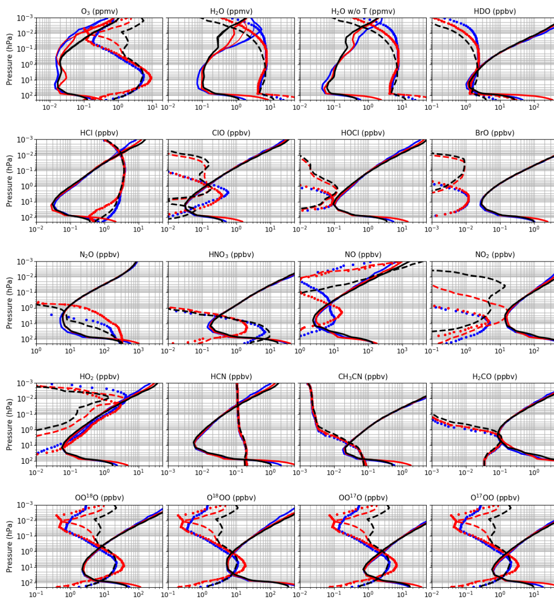
Figure 9. Single-scan retrieval precision (full lines), nighttime VMR (dashed lines) and daytime VMR (dotted lines) profiles. Profiles are shown at 80° S (blue line), Equator (red line) and 80° N (black line). The thick (thin) red full lines are nighttime (daytime) conditions. The H 2 O results without temperature retrieval are indicated by “w/o T”.
