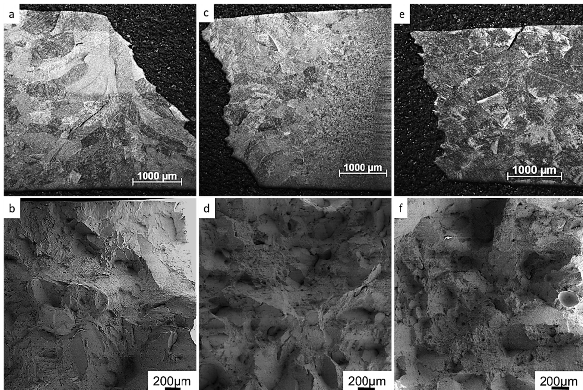
Figure 5.2. Etched side views and fracture surfaces of weld samples tensile tested at room temperate. a) and b) EBW, c) and d) LBW, and e) and f) PAW.
