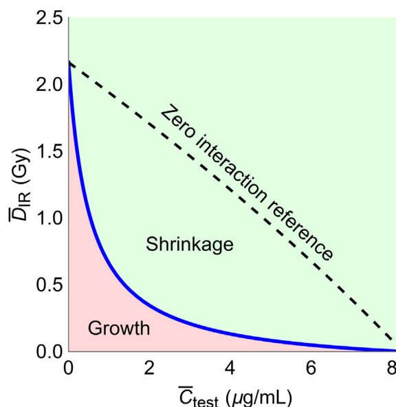
Fig. 7. The Tumor Static Exposure (TSE) curve as a function of radiation dose and radiosensitizer concentration. The set of all concentration-dose pairs that yield tumor shrinkage upon daily administration is shown in green. Concentration pairs outside this region lead to tumor growth and are shown in red. The TSE curve is shown in blue and can be compared to the case with no synergy ( b = 0 ), shown in black (dashed). The TSE curve has significant curvature due to a pronounced synergistic effect between the treatments. (For interpretation of the references to color in this figure legend, the reader is referred to the web version of this article.)
