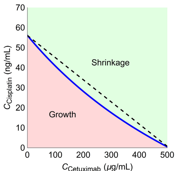
Fig. 4. The Tumor Static Concentration (TSE) curve for combinations of cetuximab and cisplatin plasma concentrations (blue, bold) separating regions of tumor growth (light red) and tumor shrinkage (light green). Reference straight line connecting the individual TSE values (black, dashed). (For interpretation of the references to color in this figure legend, the reader is referred to the web version of this article.)
