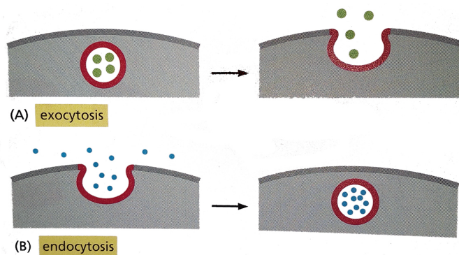
Fig 15. (a) Showing vesicle membrane bending and fusing with the cell membrane during exocytosis. (b) Internalization and budding off vesicle during endocytosis. Image from Ref. 23
