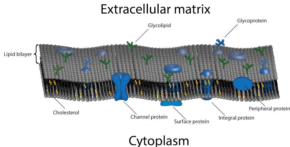
Fig.6 Simplified illustration of a cell membrane. The backbone of the membrane consists of a bilayer of lipids, within and attached to this backbone are functionalised proteins and sugar modified lipids and proteins. All carbohydrates (sugars) are located towards the extracellular matrix (outside of the cell).
