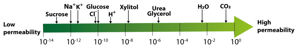
Fig.7 Showing typical permeabilities (cm/s) of some common solutes across lipid bilayers 28-31 in Log-scale. Figure adapted from 23 .
