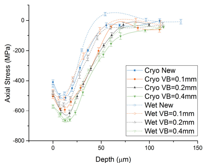
Figure 5: Residual stress profile in the axial direction (direction of feed).
