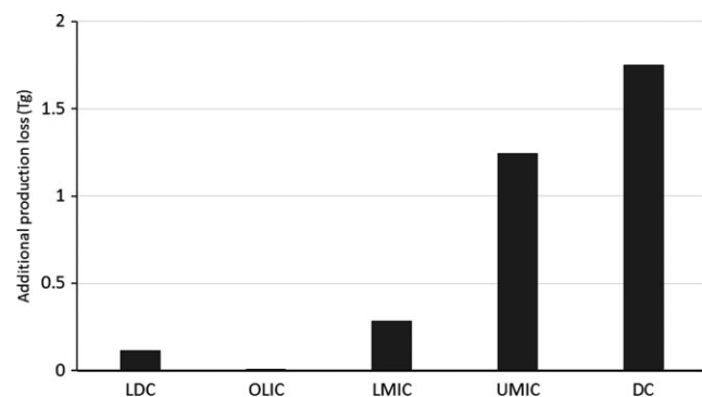
FIGURE 7 Additional lost production due to ozone, assuming 100% irrigation, presented by country category. See Figure 4 legend for key to county groupings
