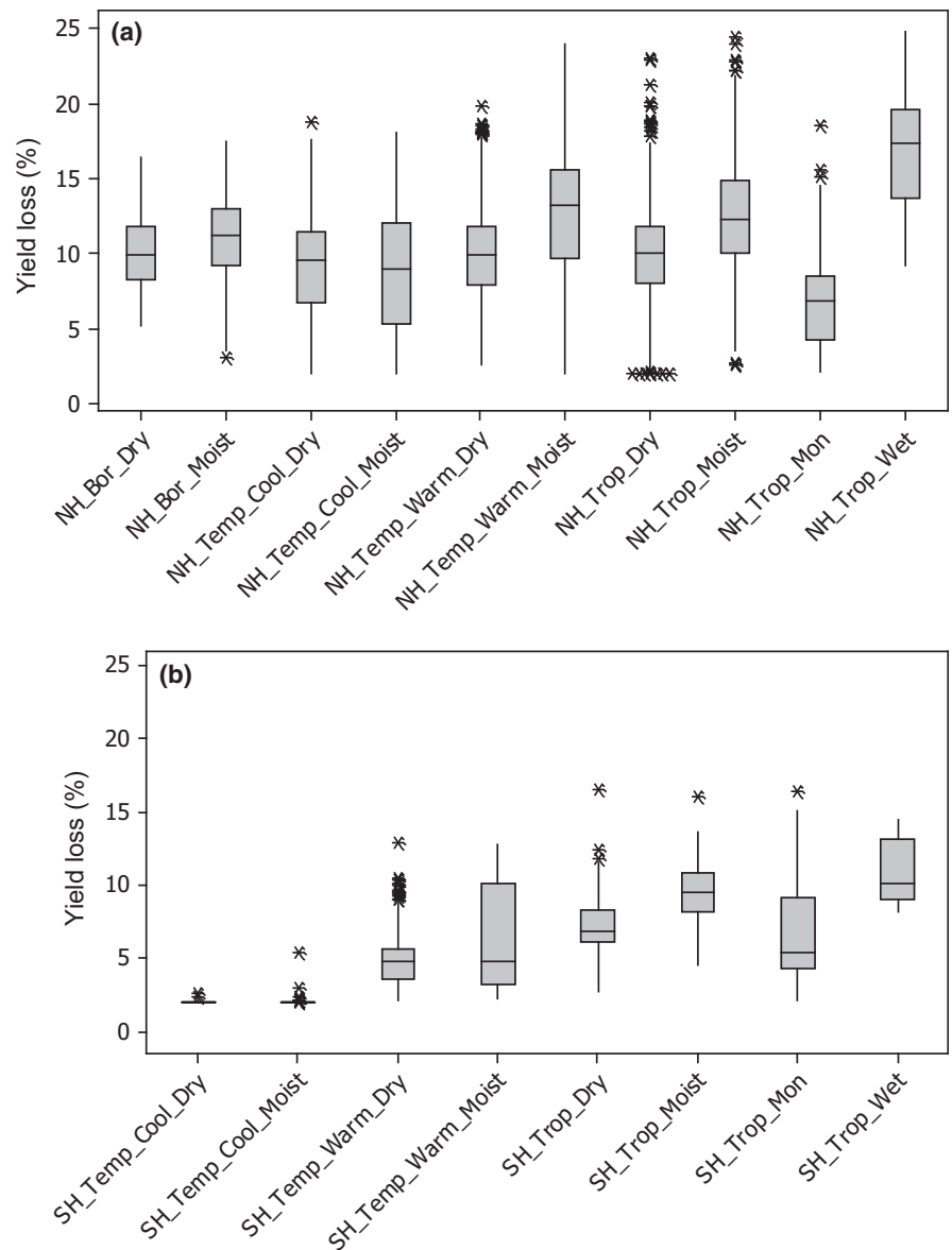
FIGURE 3 Box plot of percentage yield loss by climatic zone for the (a) northern (NH) and (b) southern hemisphere (SH), calculated using POD_3IAM as indicated in Figure 1. The box represents the interquartile range, with the top line being the third quartile (Q3), the middle line the median and the bottom line the first quartile (Q1), with the whiskers indicating the range of the data calculated as an upper limit of Q3 + 1.5(Q3 - Q1) and a lower limit of Q1 - 1.5(Q3 - Q1) , and * representing outliers
