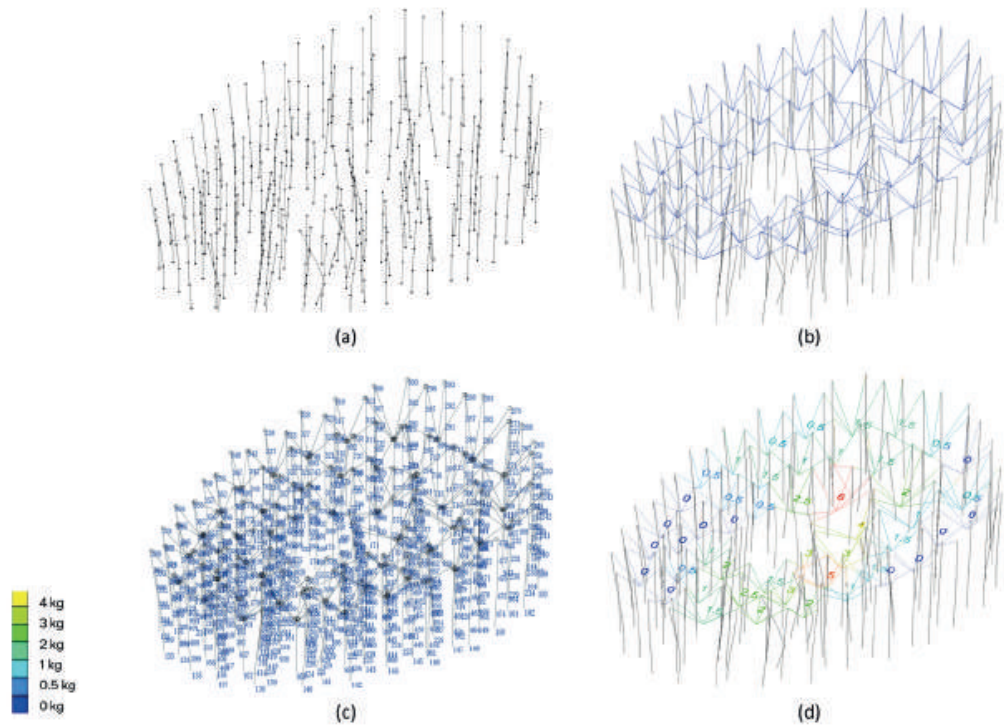
Figure 13: Structural and loading sequence optimization. (a) shows the Grasshopper generated columns based on inclination scanning. It allows mesh lines to be recreated as shown in (b). (c) displays estimated spring forces, which are used to calculate target loads and loading points for the next day (see subfigure (d)).
