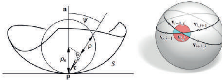
Figure 4: Left: Meusnier's theorem, relating the curvature of a curve c passing through p to normal curvature at p in direction of c' . Right: Spherical vertex star.
