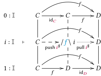
Fig. 2. Formation and elimination of /f \setminus i using Weld. The middle row depends on i and reduces to the top/bottom row when i equals 0/1. Welding produces /f \setminus i and the dashed lines.
