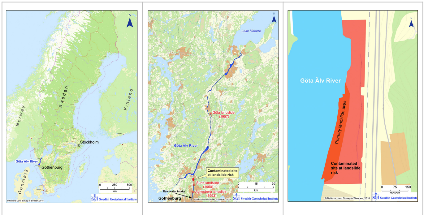
Fig. 3. Left: Map of Sweden with the Göta Älv River. Middle: The Göta Älv River and the locations: Surte 2:38, three historical landslides, and the raw water intake. Right: The Göta Älv River and the location of the study site Surte 2:28.
