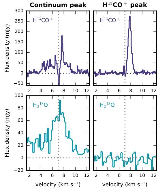
Fig. 4. Spectra extracted in a beam toward the continuum peak position (left panels) and the \text{H}^{13}\text{CO}^+ peak position ( \sim 2'' NE of the continuum peak, right panels). The top panels show the \text{H}^{13}\text{CO}^+ J = 3 - 2 transition and the bottom panels show the \text{H}_2^{18}\text{O} 3_{1,3} - 2_{2,0} transition. The two spectra for each species are shown on the same vertical scale. The systemic velocity is indicated by the vertical dotted line at v_{\text{lsr}} \approx 7 km s ^{-1} .
