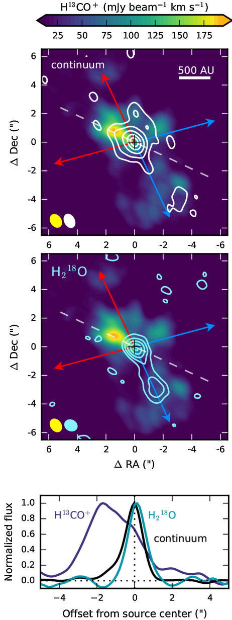
Fig. 2. Integrated intensity map for the \text{H}^{13}\text{CO}^+ J = 3 - 2 transition (color scale) toward IRAS2A. The 1.2 mm continuum is overlaid in white contours (top panel) and the \text{H}_2^{18}\text{O} 3_{1,3} - 2_{2,0} transition in blue contours (middle panel). The continuum contours are 1.8 (1\sigma) \times [3, 10, 25, 50, 75] mJy beam ^{-1} , and the \text{H}_2^{18}\text{O} contours are 9.8 (1\sigma) \times [3, 8, 15, 25, 35] mJy beam ^{-1} km s ^{-1} . The beams are depicted in the bottom left corner. The position of the continuum peak is indicated by a black cross (the close binary is unresolved in these data) and the outflow axes by red and blue arrows. The integrated intensities along the dashed white line are shown in the bottom panel, normalized to their maximum value. The zero flux level and source position are indicated by dotted lines.
