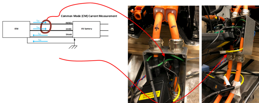
Figure 11.5 - Measurement of CM current using a common probe for positive and negative directions.
