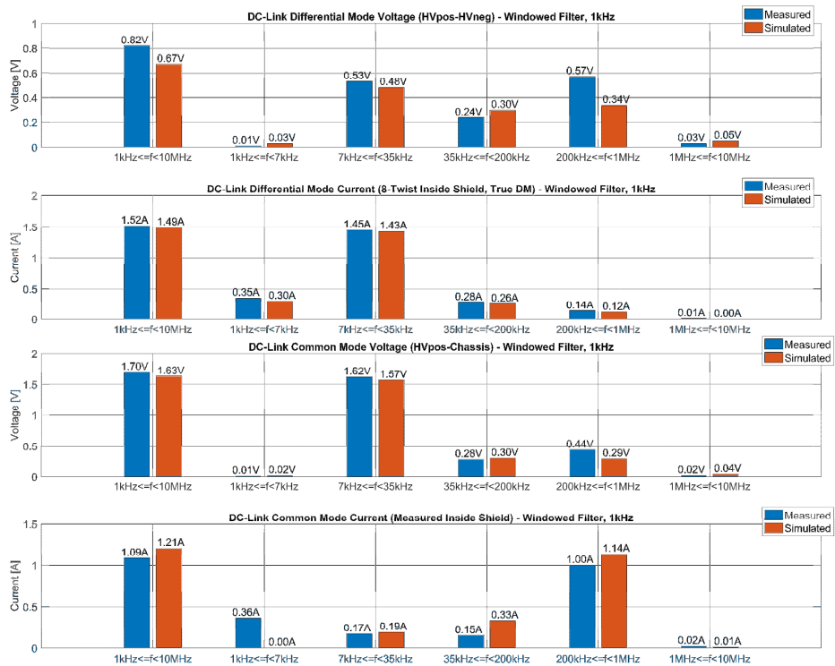
Figure 11.13 - DC link results using rms values in frequency bands.
