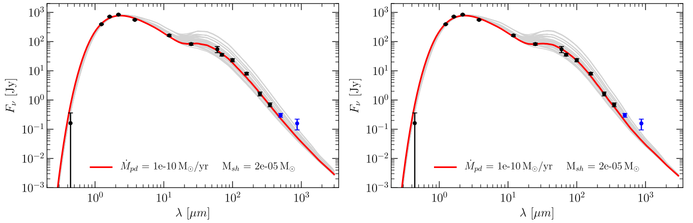
Fig. A.1. Model grids calculated with opacities by Zubko et al. (1996) ( left ) and Preibisch et al. (1993) ( right ) for 0.1 \mu\text{m} solid, spherical amC dust grains in a present-day wind and detached shell. The best-fitting model is represented with a solid red line, and the respective best-fitting model parameters are given in the legend. The grey lines represent the other models in the grid.
