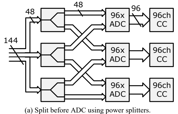
(a) Split before ADC using power splitters.
