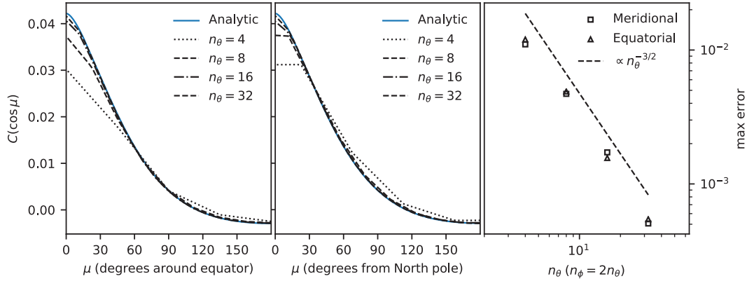
Figure 3: Error analysis for an example GMRF. The left and middle panels estimate the covariance along equatorial and meridional lines, respectively, and the analytic covariance in blue. The right panel indicates the convergence of the error as a function of n_\theta .
