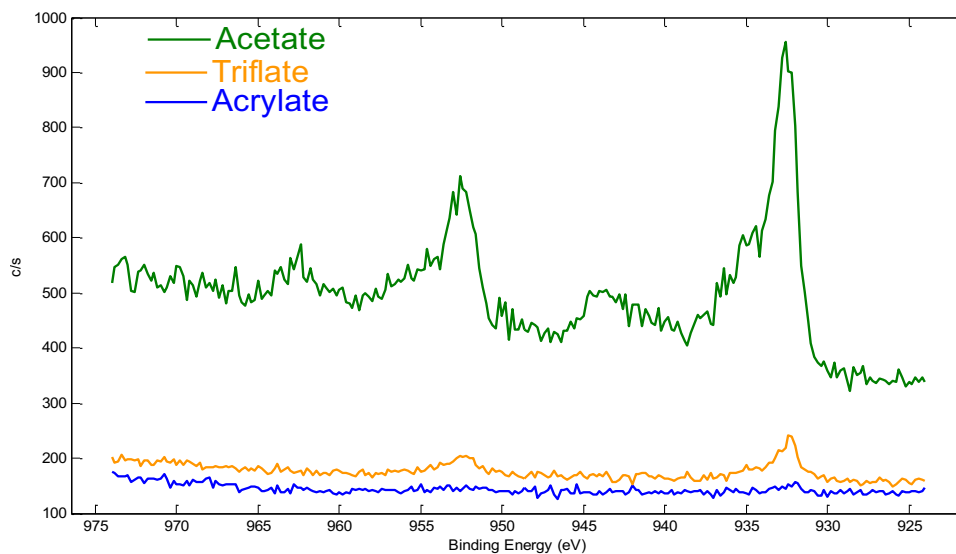
Figure 39. High resolution XPS spectra of the Cu_{2p3} region for 6-OAc, 5-OTf, and 7-Acryl.
