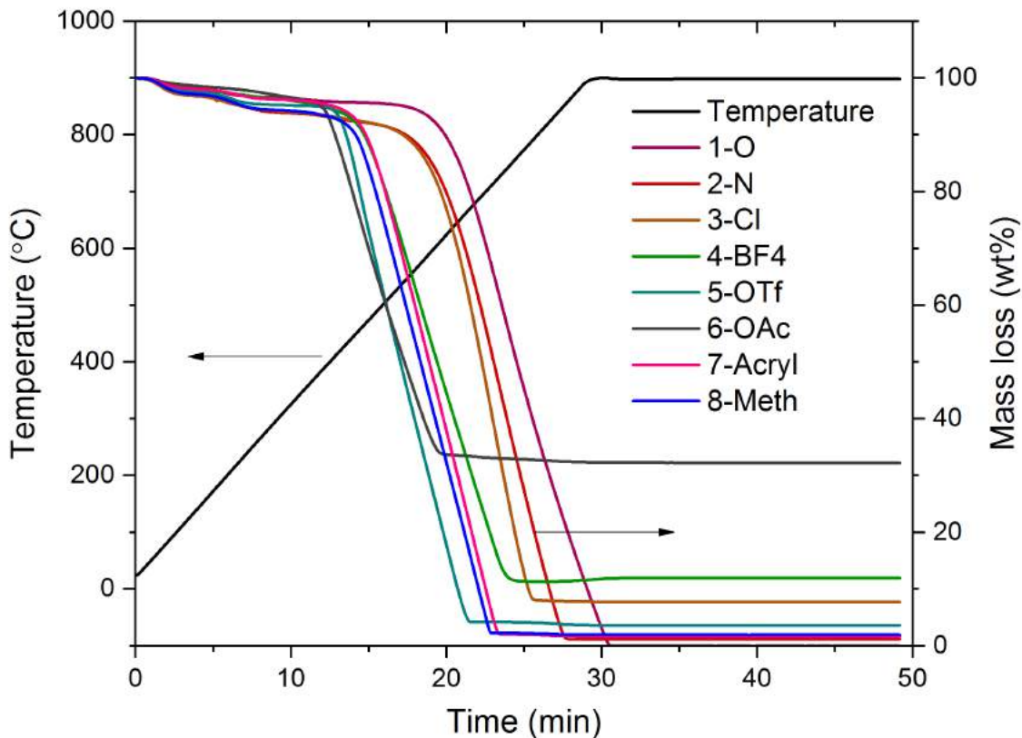
Figure 38. Thermograms of OMCs ran under air. The final masses correspond to copper loadings.
