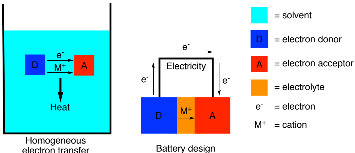
Figure 9. Comparison of homogeneous electron transfer (left) vs. battery design (right) between the donor ( D ) and acceptor ( A ). In homogenous electron transfer, both the electrons ( e^- ) and cations ( M^+ ) travel the same path and the energy change, \Delta G , is released as heat. In contrast, in the battery architecture, the electrons and cations take different paths and most of the energy is captured as electricity.
