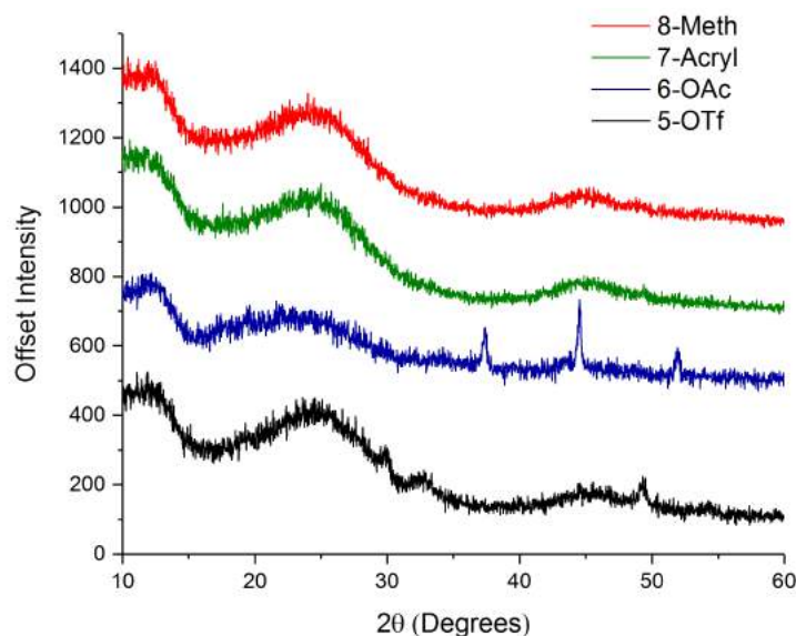
Figure 37. X-ray diffractograms of 5-OTf, 6-OAc, 7-Acryl, and 8-Meth Cu-OMCs
