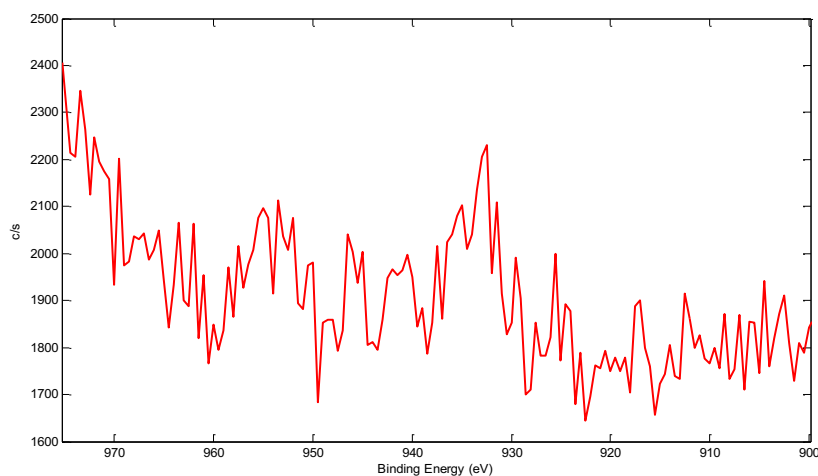
Figure 40. Spectrum of the Cu_{2p3} region for 4-BF4.
