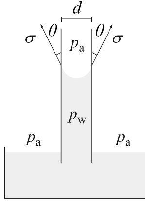
Figure 3.2: The capillary rise is due to the surface tension between gas and liquid phases. The capillary pressure in a narrow tube can be expressed from force equilibrium as p^c = p^a - p^w = 4\sigma \cos\theta/d . For further discussions about the capillary effect, see [56].
