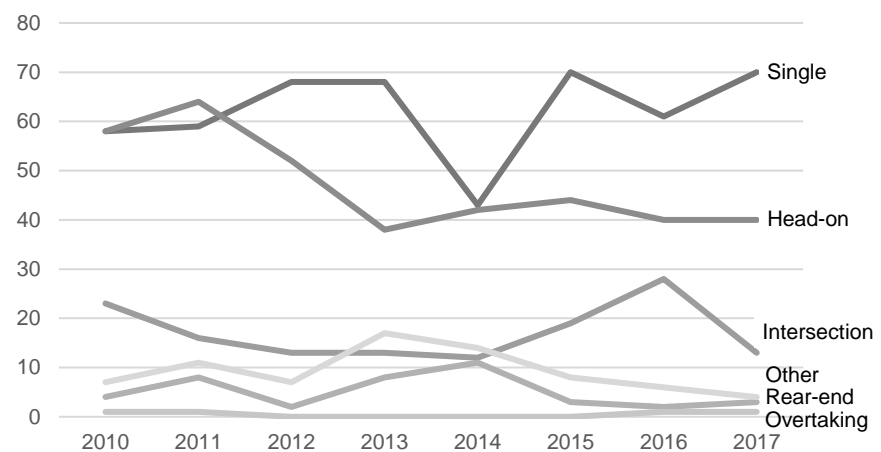
Figure 5: Passenger car occupant fatalities in Sweden during 2010-2017 (Trafikanalys 2018).
