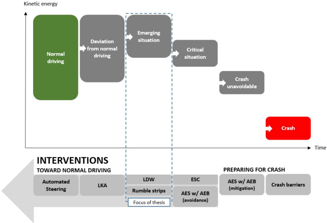
Figure 9: Focus of thesis and LDW in the integrated safety chain, adopted from Tingvall (2008), Lie (2012b) and Strandroth (2015). Detectable lanes is a precondition for lane keeping. Autonomous Emergency Braking is referred to as AEB.
