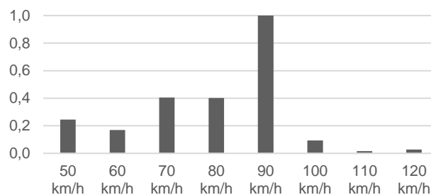
Figure 6: Head-on fatalities per traffic volume (vehicle kilometre) in relation to 90 km/h roads. Data extracted from STRADA and the national road database (NVDB) 2010-2016.
