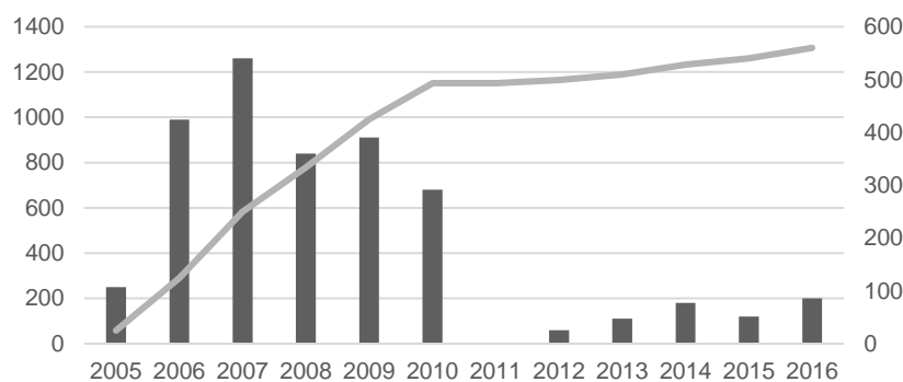
Figure 8: Implemented milled centreline rumble strips on two-lane roads in Sweden (km) and corresponding accumulated levels, adapted from Swedish Transport Administration (2017).
