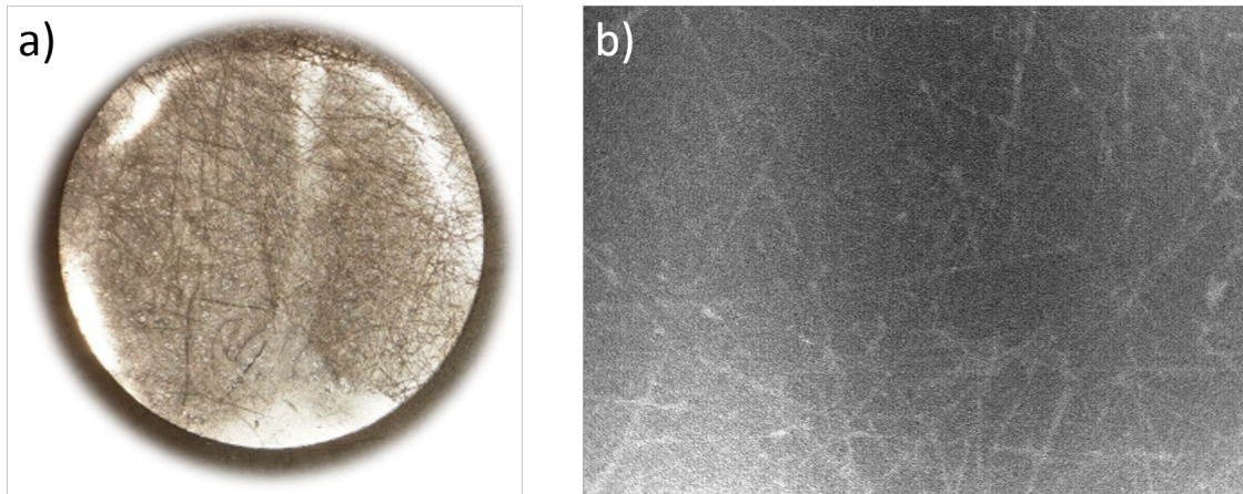
Figure 3.3: a) Photo of the infiltrated CF-SMFC preform. b) X-ray image of the assembled TIM sandwich structure.
