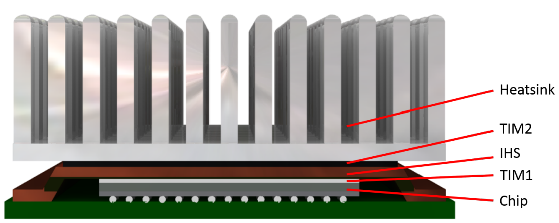
Figure 2.2: A typical BGA package with TIMs between chip and internal heat spreader (IHS), and between IHS and heatsink.
