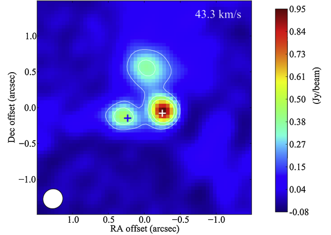
Fig. 2. ALMA observations of CO( 3-2 ) towards the Mira AB system at v_{\text{LSR}} = 43.3 km s -1 . The white and blue plus symbols show the positions of omi Cet (Mira A) and VZ Cet (Mira B), respectively. The contours are overlaid on the image with 20, 35, and 50% of the peak value. The observed CI emission likely arises from the region near Mira B. The beam is shown in the lower left corner.
