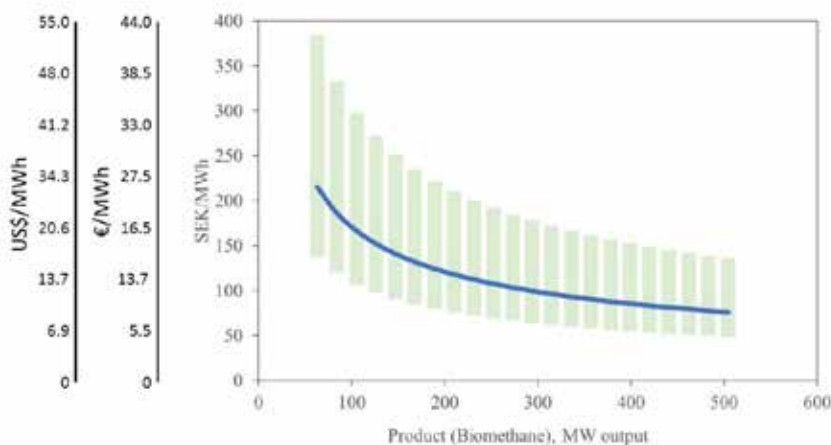
Figure 4: Depreciation cost for biomethane including non-technical uncertainties divided by the expected production during the technical lifetime of the plant (20 years). Exchange rates: 9.1 SEK per 1.0 € (average exchange rate during the project) and 1.25 US$ per 1.0 €.
