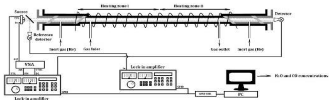
THz experimental setup. Figure: Hosein Bidgoli.
