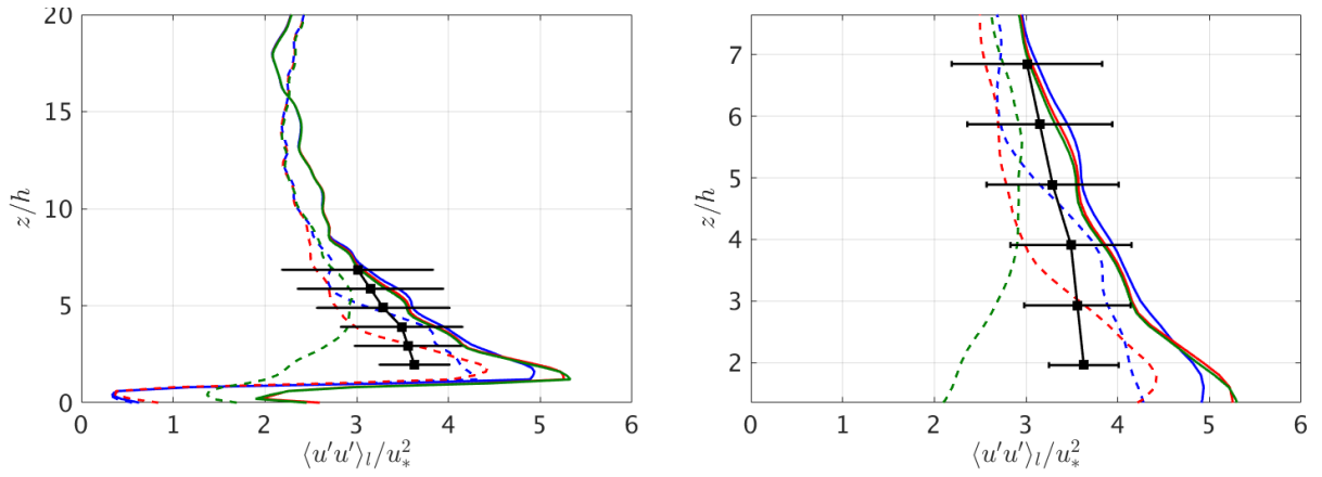
Figure 2.8: \langle u'u' \rangle_l / u_*^2 from atmospheric boundary layer simulations at location of the wind turbine to the left and a zoom in rotor plane to the right. — : Wind turbine 1 in homogeneous forest, - - : Wind turbine 2 in homogeneous forest, — : Wind turbine 1 in current clearing, - - : Wind turbine 2 in current clearing, — : Wind turbine 1 in extended clearing, - - : Wind turbine 2 in extended clearing, ■ : Measurements
