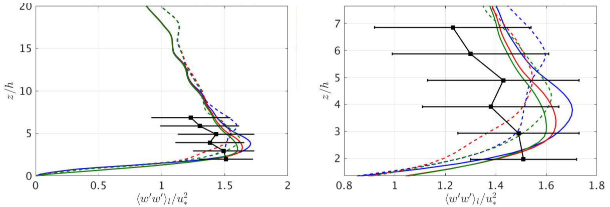
Figure 2.10: \langle w'w' / u_*^2 \rangle from atmospheric boundary layer simulations at location of the wind turbine to the left and a zoom in rotor plane to the right. —: Wind turbine 1 in homogeneous forest, - - : Wind turbine 2 in homogeneous forest, —: Wind turbine 1 in current clearing, - - : Wind turbine 2 in current clearing, —: Wind turbine 1 in extended clearing, - - : Wind turbine 2 in extended clearing, ■: Measurements
