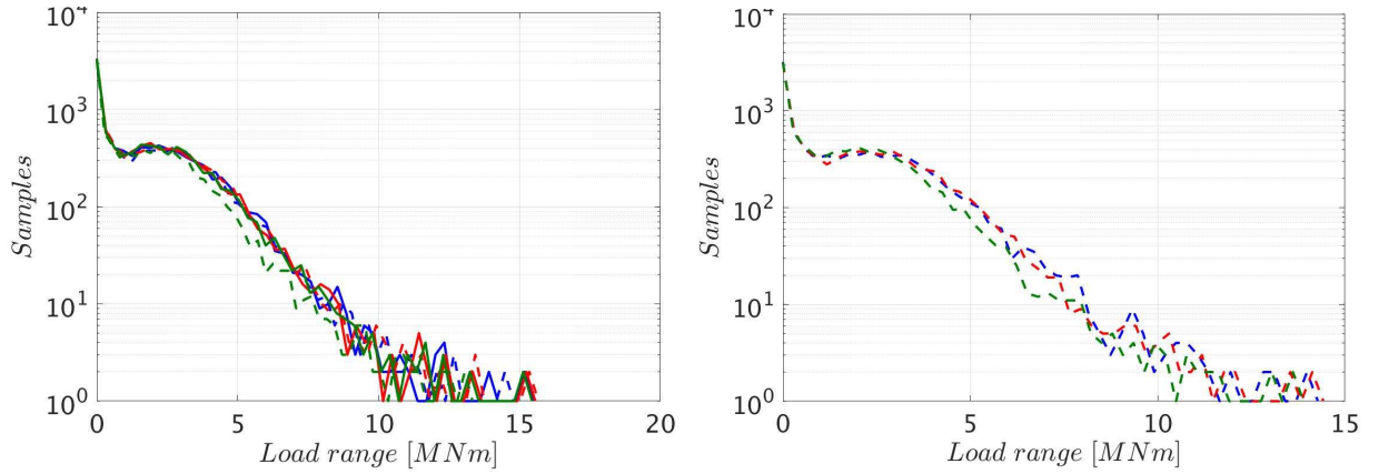
Figure 2.16: Rain flow of yaw bearing moment around the y-axis. Both wind turbines to the left and only wind turbine 2 to the right. — : Wind turbine 1 in homogeneous forest, - - : Wind turbine 2 in homogeneous forest, — : Wind turbine 1 in current clearing, - - : Wind turbine 2 in current clearing, — : Wind turbine 1 in extended clearing, - - : Wind turbine 2 in extended clearing
