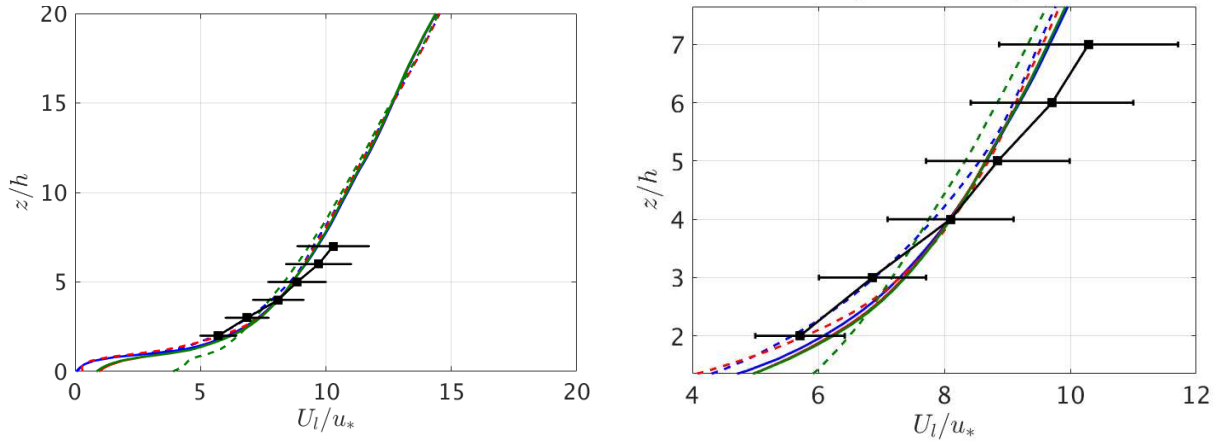
Figure 2.5: \langle U_l/u_* \rangle from atmospheric boundary layer simulations at location of the wind turbine to the left and a zoom in rotor plane to the right. —: Wind turbine 1 in homogeneous forest, - -: Wind turbine 2 in homogeneous forest, —: Wind turbine 1 in current clearing, - -: Wind turbine 2 in current clearing, —: Wind turbine 1 in extended clearing, - -: Wind turbine 2 in extended clearing, ■: Measurements
