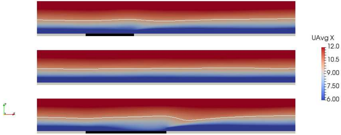
Figure 2.3: Time averaged \bar{u} velocity in atmospheric boundary layer simulations on plane at y of 400m. Contour line in white shows time averaged \bar{u} velocity of 10m/s. From the top current clearing, homogeneous forest and extended clearing. Below each plane the location of the clearing is marked in black.
